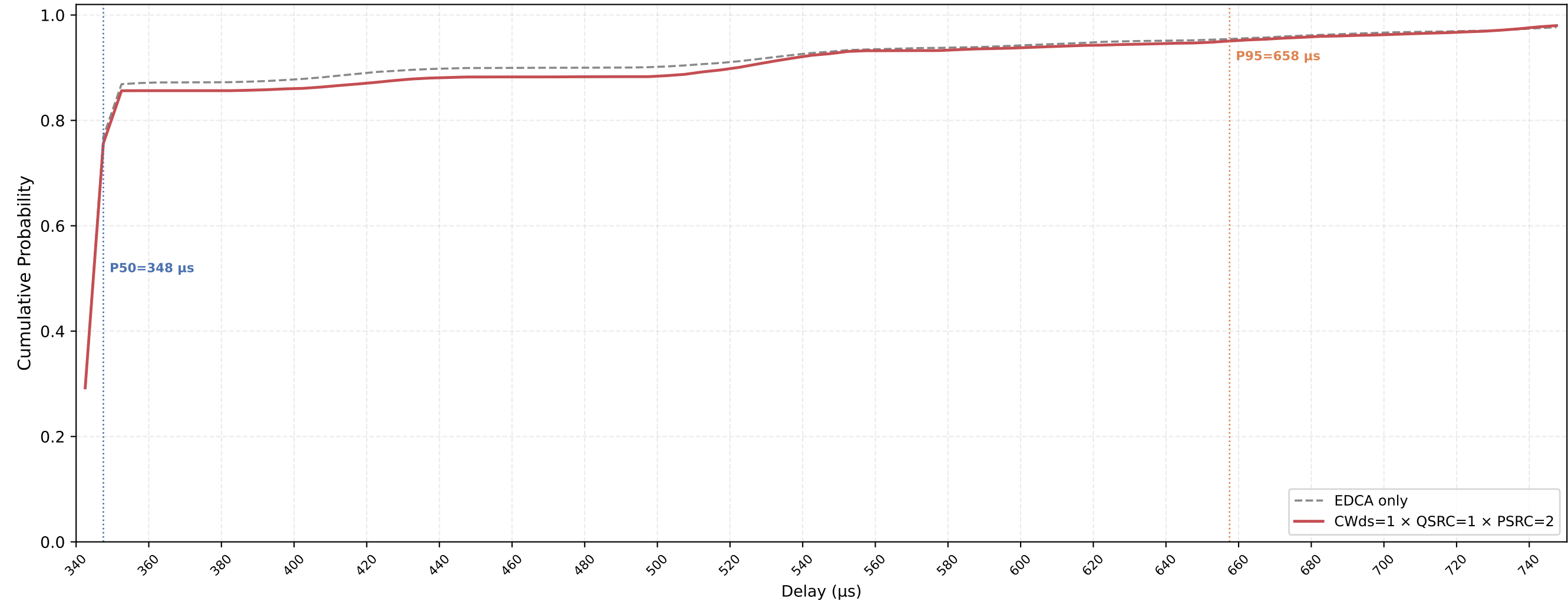
Legacy STA VO Delay CDF — CWds=1 × QSRC=1 × PSRC=2 nSta=30, nPedca=15, 0.1Mbps, avg of 10 runs
