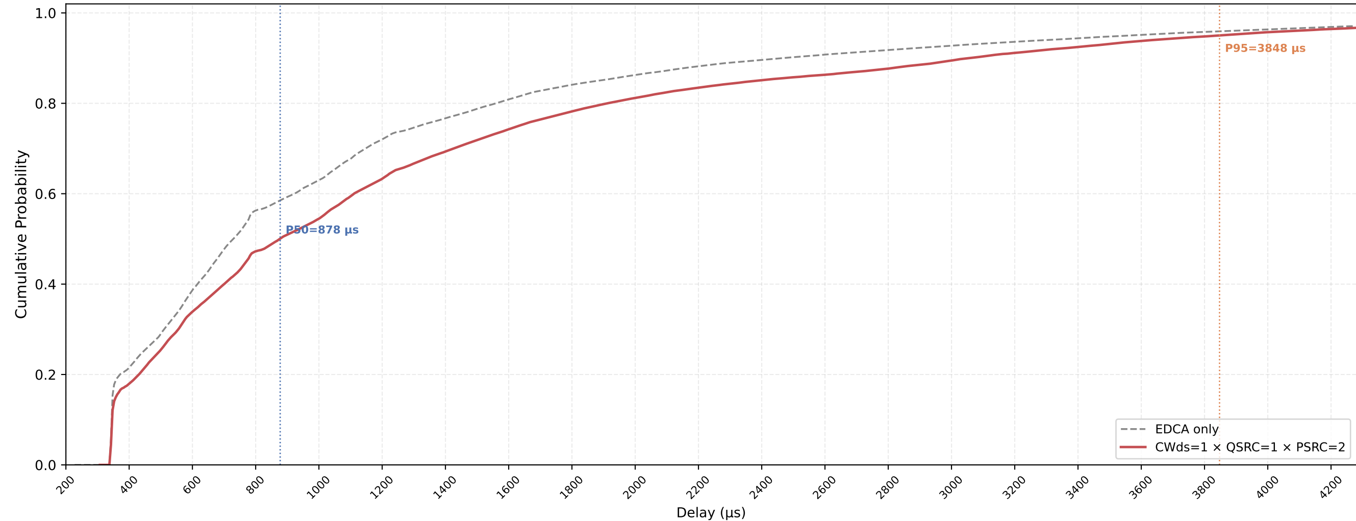
P-EDCA STA VO Delay CDF — CWds=1 × QSRC=1 × PSRC=2 nSta=30, nPedca=15, 0.5Mbps, avg of 10 runs
