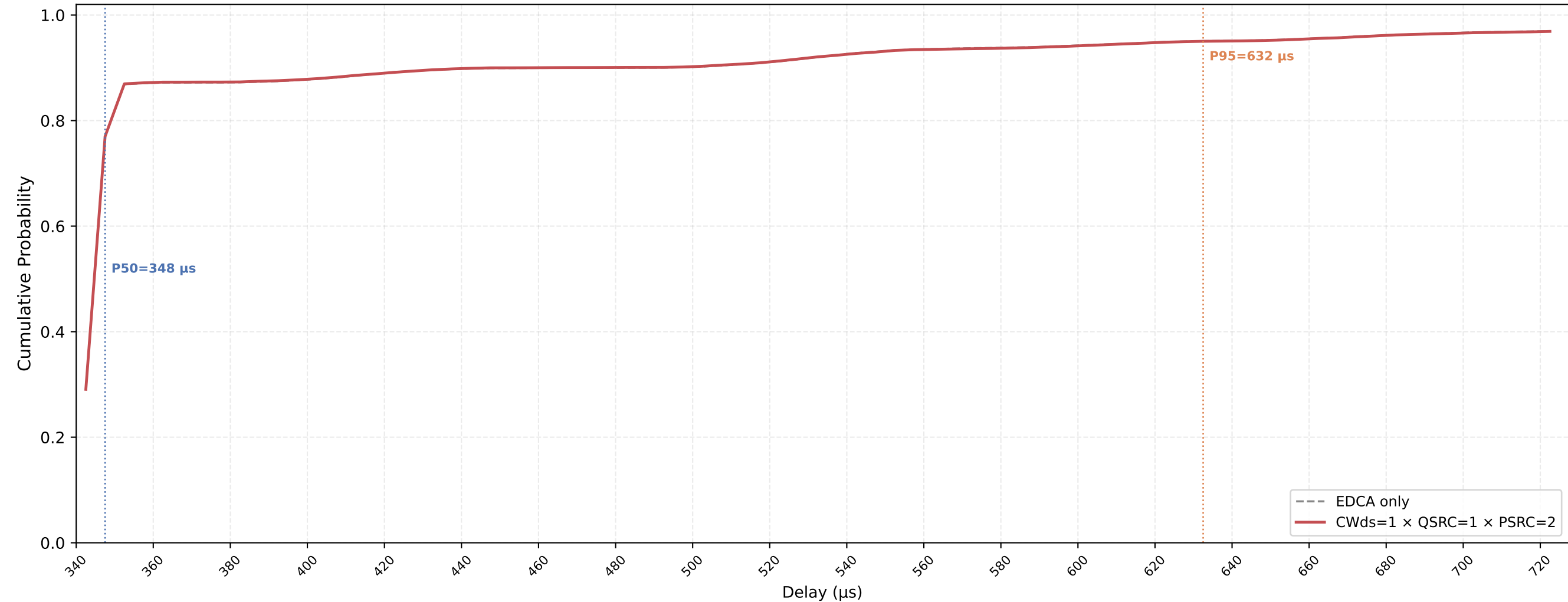
VO (all STAs) Delay CDF — CWds=1 × QSRC=1 × PSRC=2 nSta=30, nPedca=5, 0.1Mbps, avg of 10 runs
