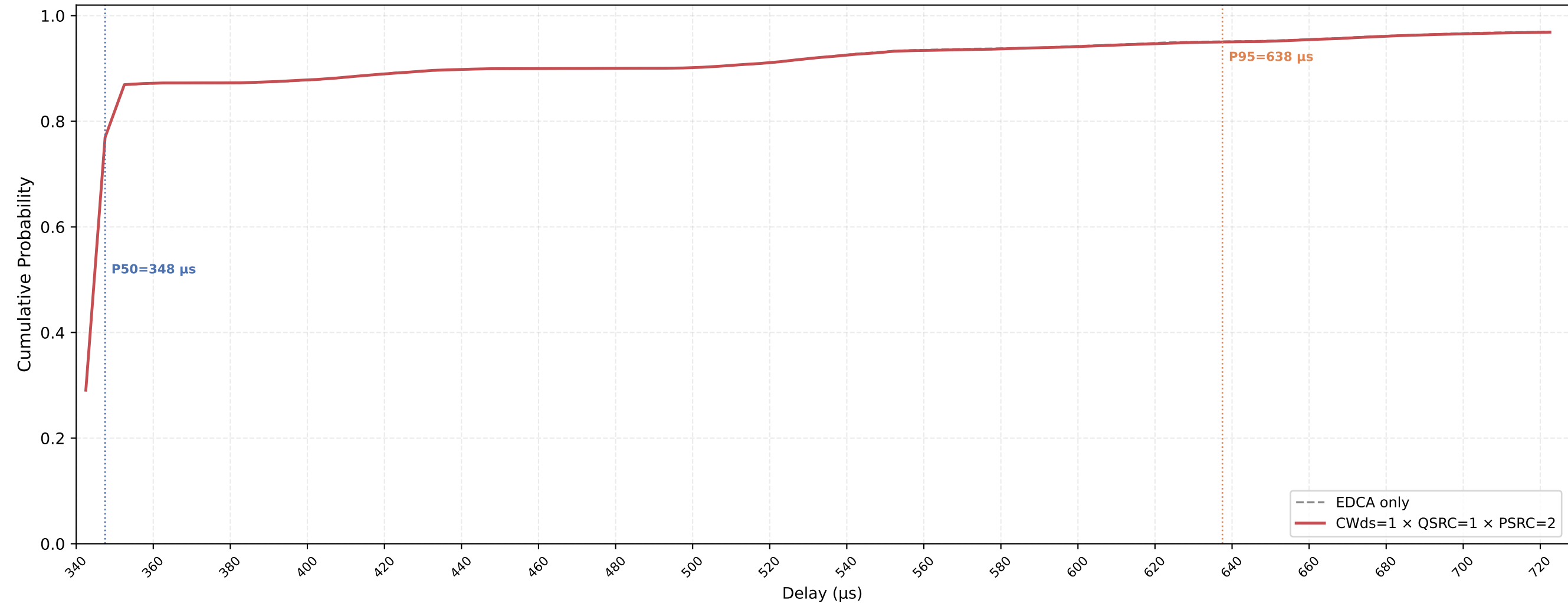
VO (all STAs) Delay CDF — CWds=1 × QSRC=1 × PSRC=2 nSta=30, nPedca=15, 0.1Mbps, avg of 10 runs
