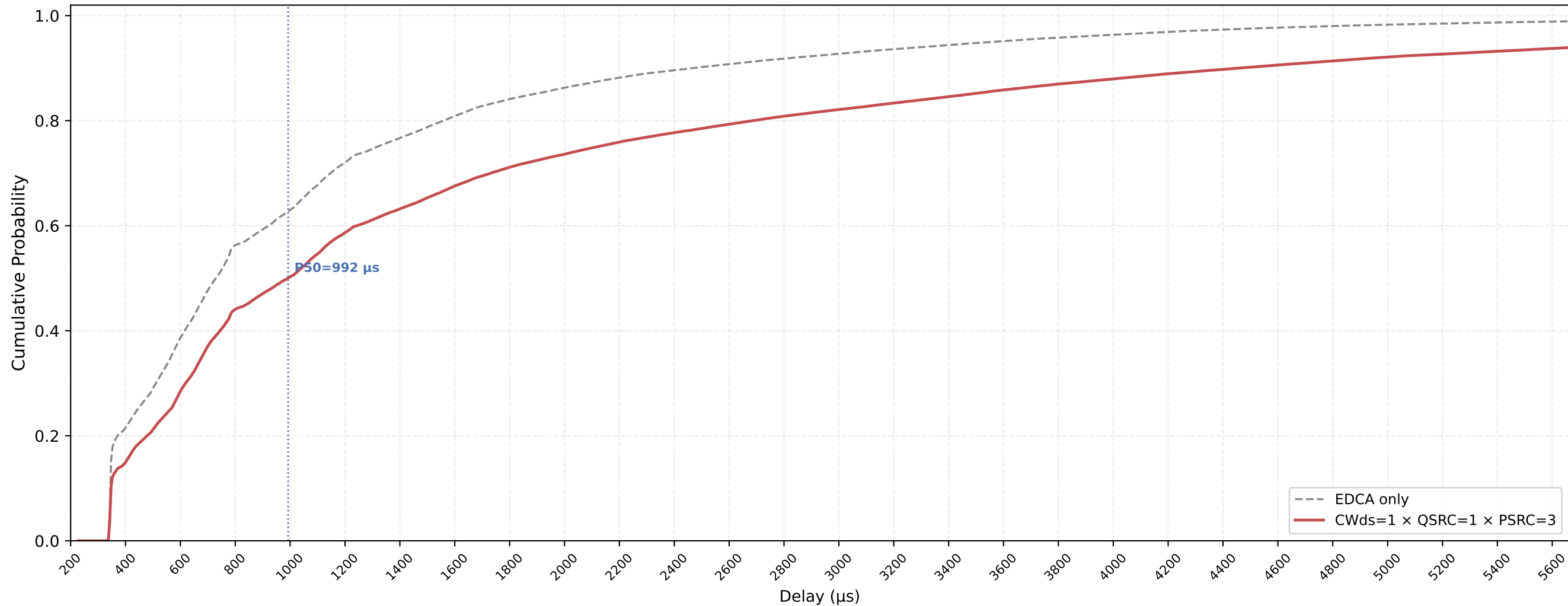
Legacy STA VO Delay CDF — CWds=1 × QSRC=1 × PSRC=3 nSta=30, nPedca=15, 0.5Mbps, avg of 10 runs
