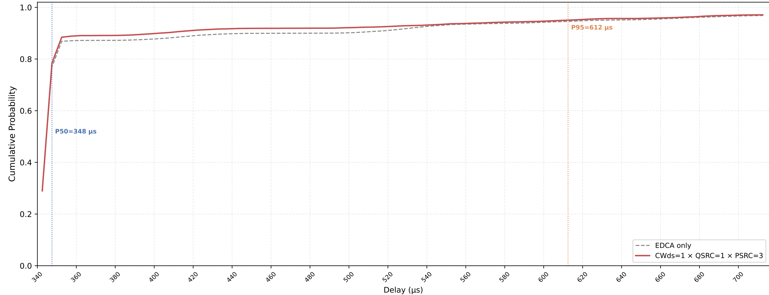
P-EDCA STA VO Delay CDF — CWds=1 × QSRC=1 × PSRC=3 nSta=30, nPedca=15, 0.1Mbps, avg of 10 runs
