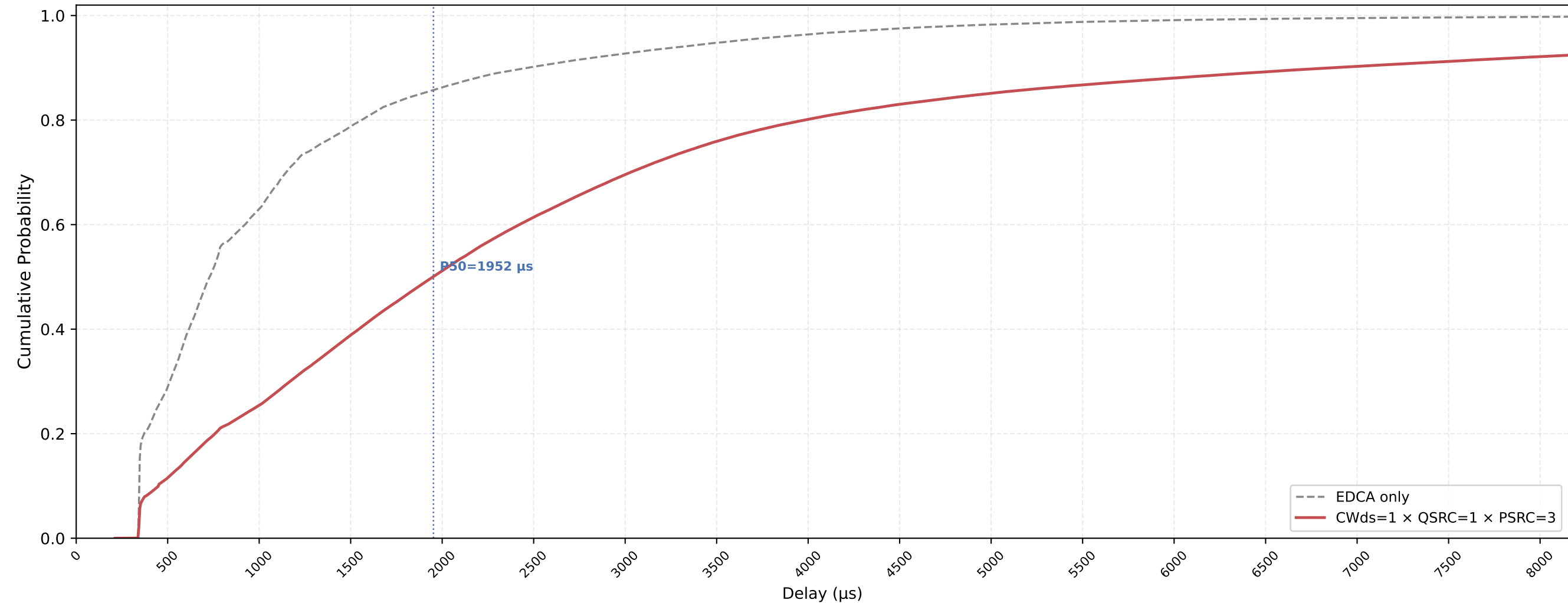
VO (all STAs) Delay CDF — CWds=1 × QSRC=1 × PSRC=3 nSta=30, nPedca=30, 0.5Mbps, avg of 10 runs
