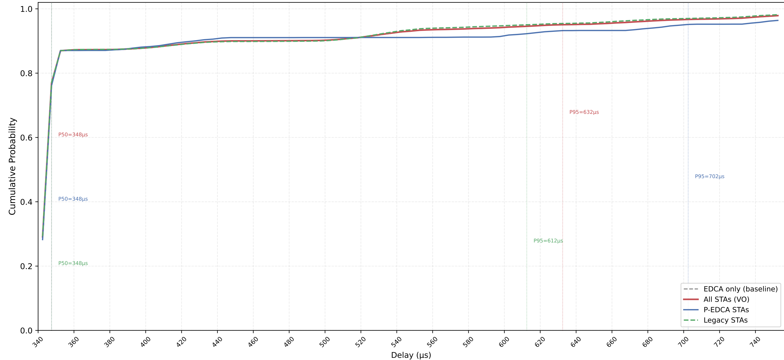
VO Delay CDF — P-EDCA / Legacy / All | CWds=1 × QSRC=2 × PSRC=2 nSta=30, nPedca=5/30, 0.1Mbps, avg of 10 runs
