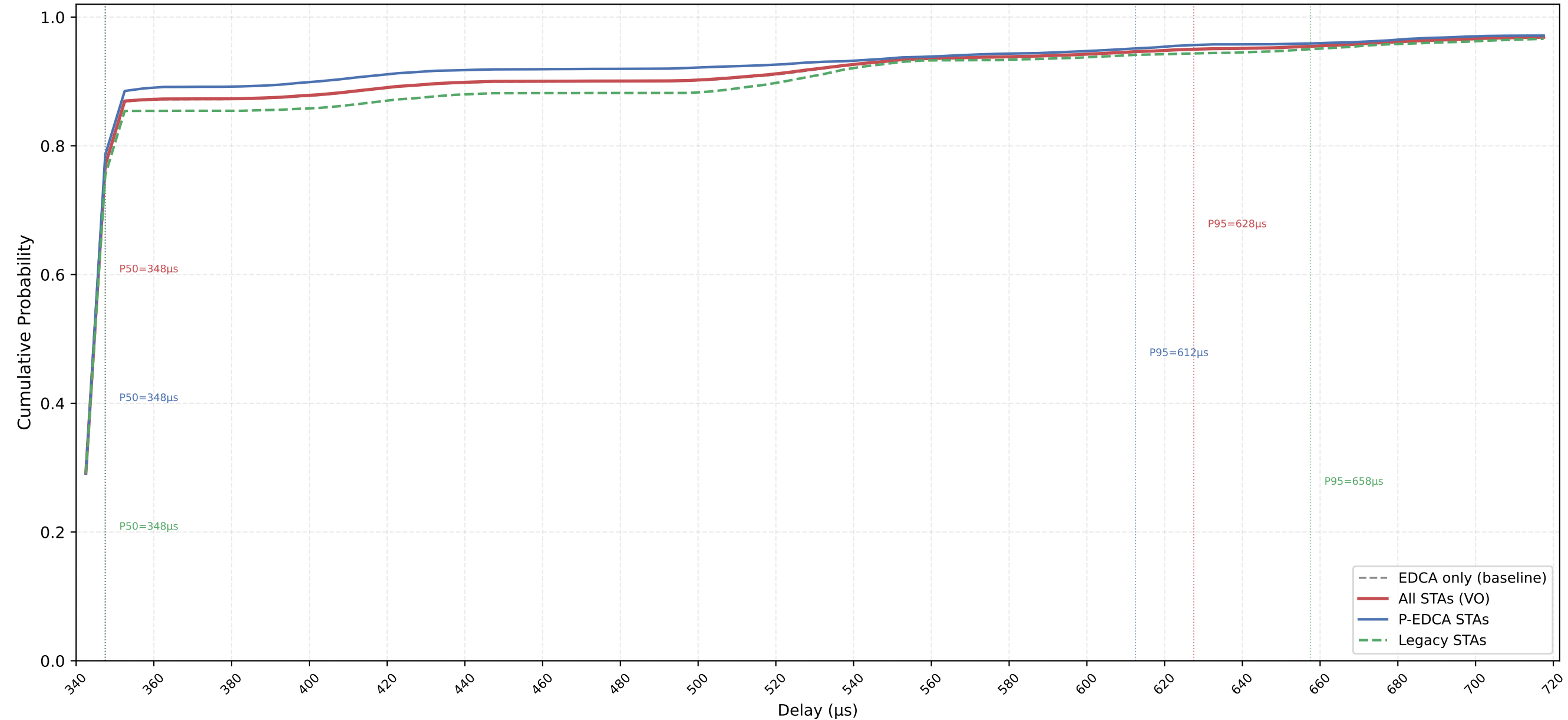
VO Delay CDF — P-EDCA / Legacy / All | CWds=1 × QSRC=2 × PSRC=2 nSta=30, nPedca=15/30, 0.1Mbps, avg of 10 runs
