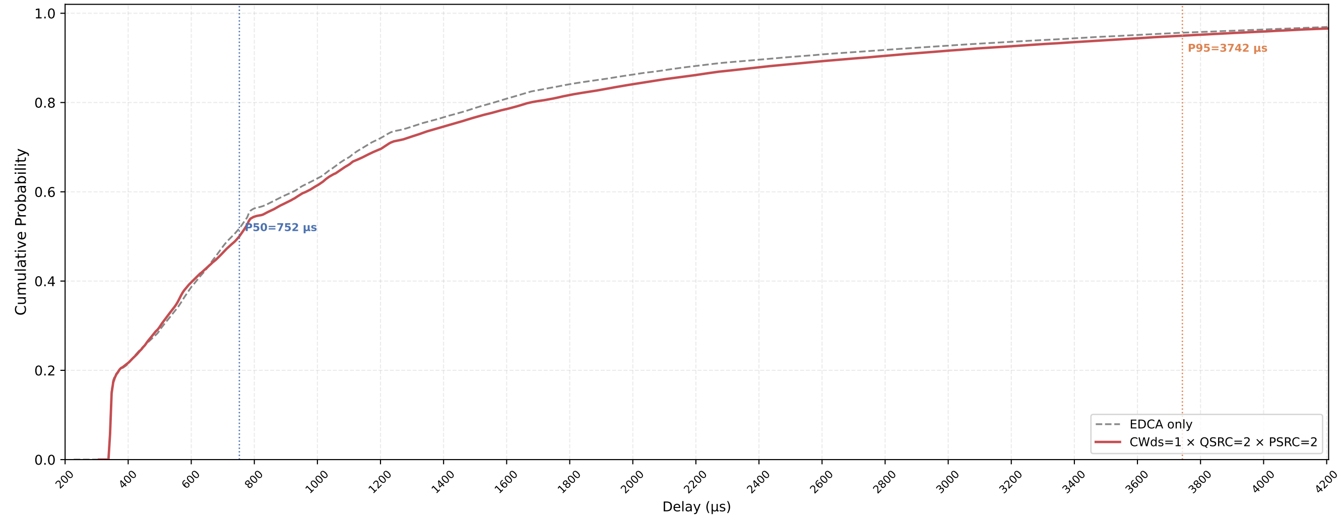
P-EDCA STA VO Delay CDF — CWds=1 × QSRC=2 × PSRC=2 nSta=30, nPedca=15, 0.5Mbps, avg of 10 runs
