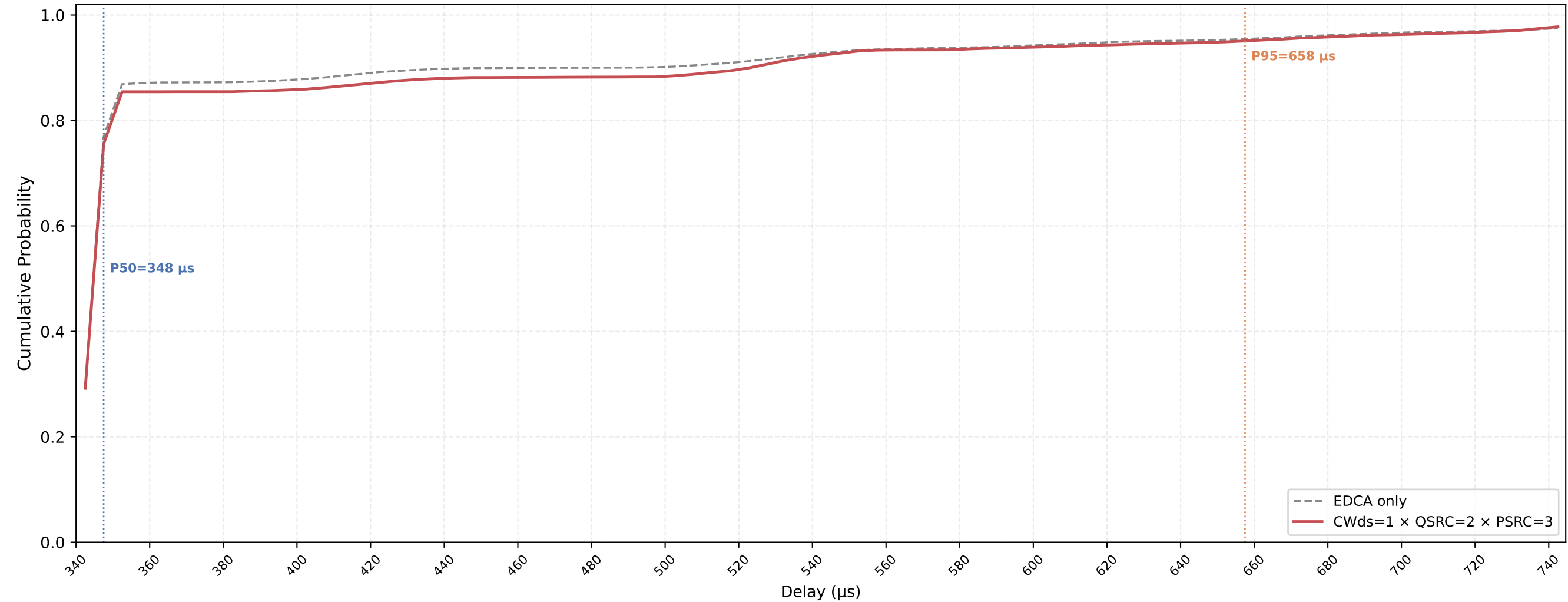
Legacy STA VO Delay CDF — CWds=1 × QSRC=2 × PSRC=3 nSta=30, nPedca=15, 0.1Mbps, avg of 10 runs
