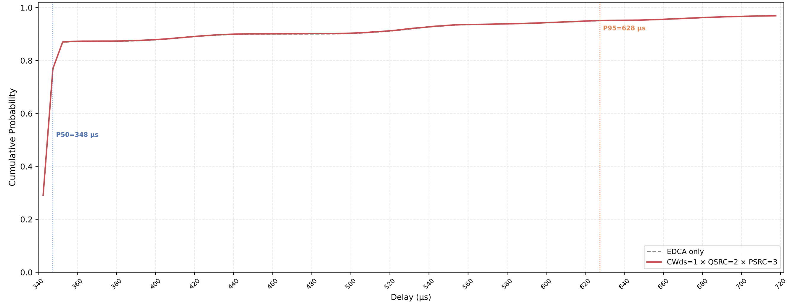
VO (all STAs) Delay CDF — CWds=1 × QSRC=2 × PSRC=3 nSta=30, nPedca=5, 0.1Mbps, avg of 10 runs
