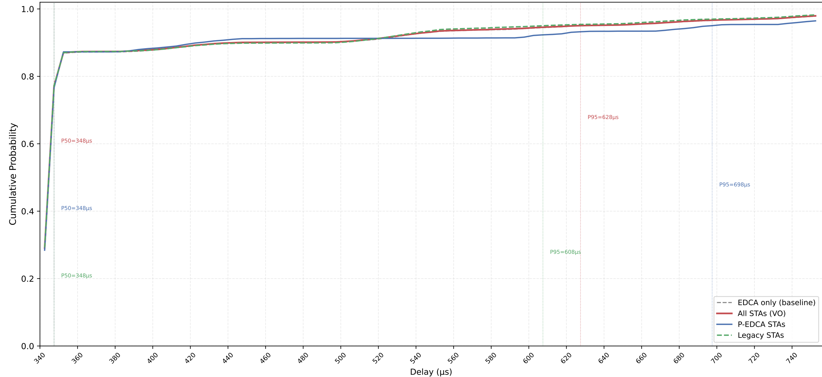
VO Delay CDF — P-EDCA / Legacy / All | CWds=1 × QSRC=3 × PSRC=2 nSta=30, nPedca=5/30, 0.1Mbps, avg of 10 runs
