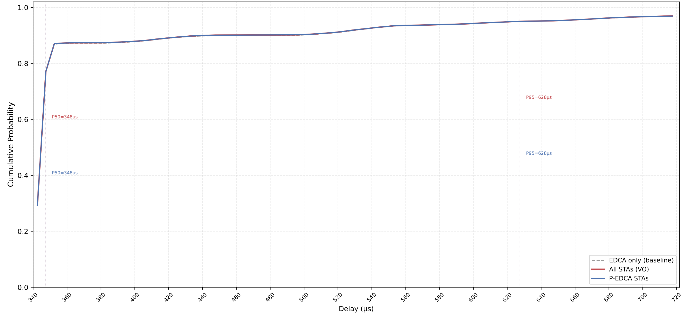
VO Delay CDF — P-EDCA / Legacy / All | CWds=1 × QSRC=3 × PSRC=2 nSta=30, nPedca=30/30, 0.1Mbps, avg of 10 runs
