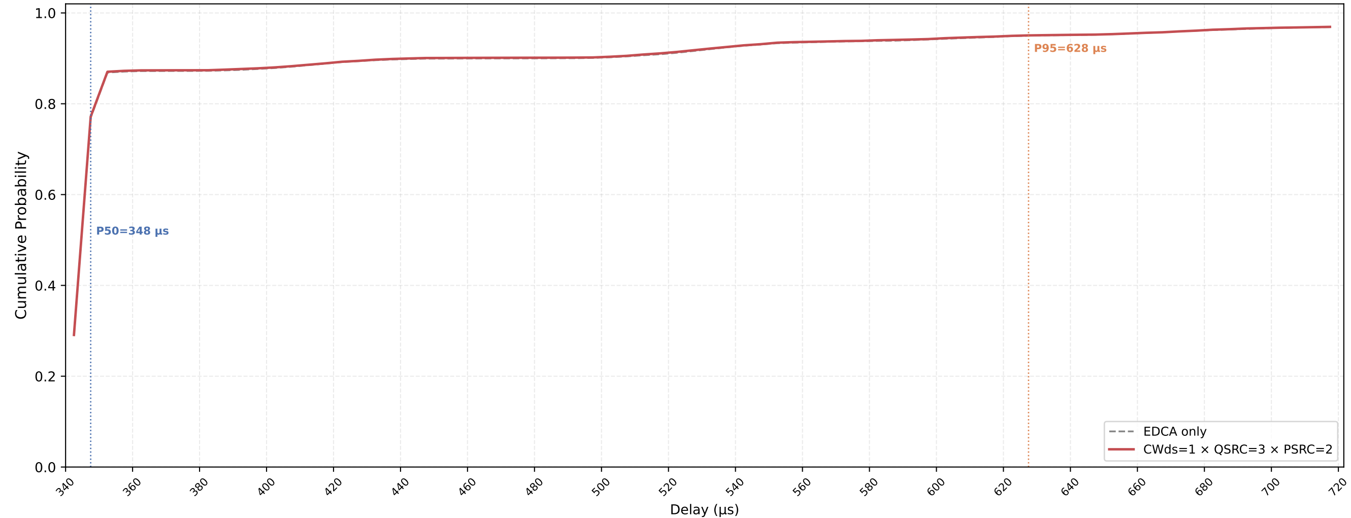
VO (all STAs) Delay CDF — CWds=1 × QSRC=3 × PSRC=2 nSta=30, nPedca=5, 0.1Mbps, avg of 10 runs
