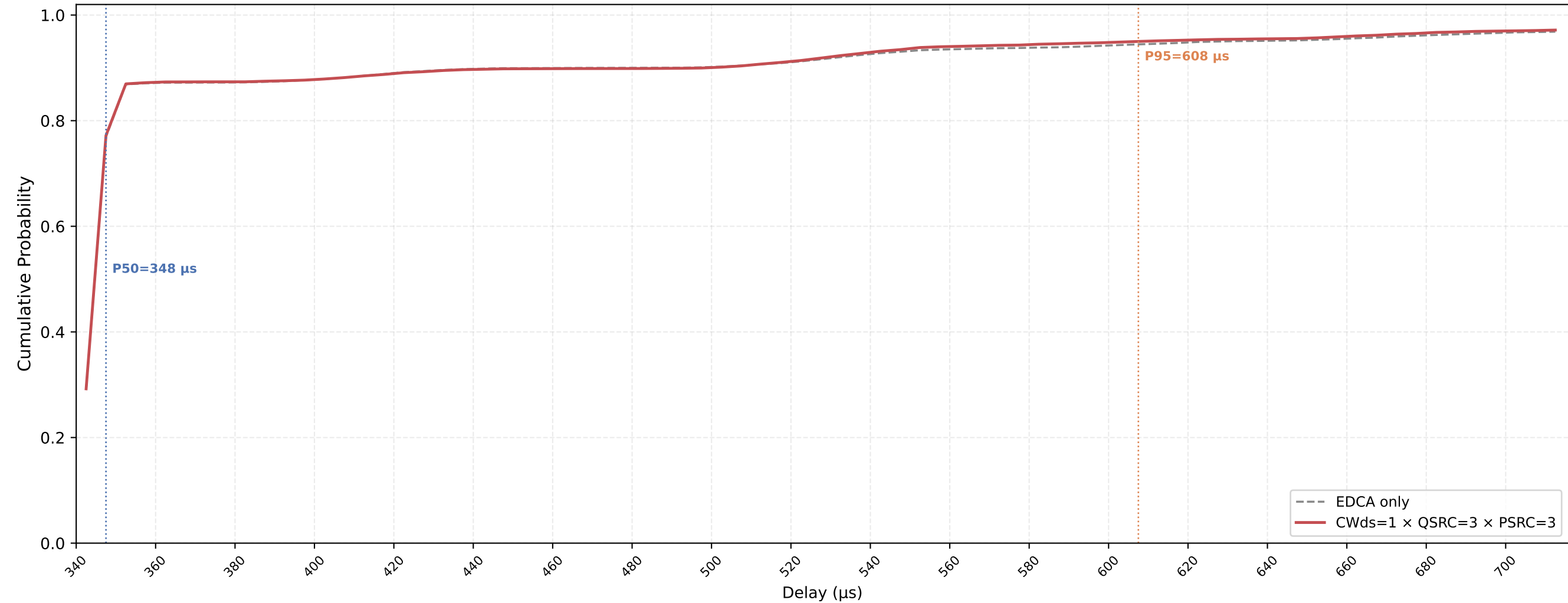
Legacy STA VO Delay CDF — CWds=1 × QSRC=3 × PSRC=3 nSta=30, nPedca=5, 0.1Mbps, avg of 10 runs
