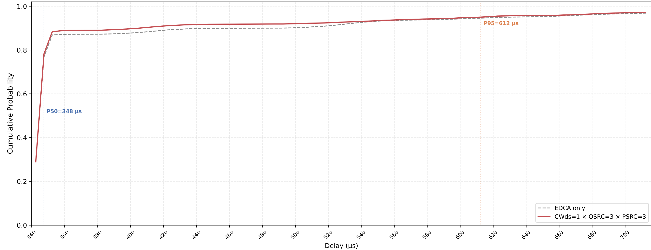
P-EDCA STA VO Delay CDF — CWds=1 × QSRC=3 × PSRC=3 nSta=30, nPedca=15, 0.1Mbps, avg of 10 runs
