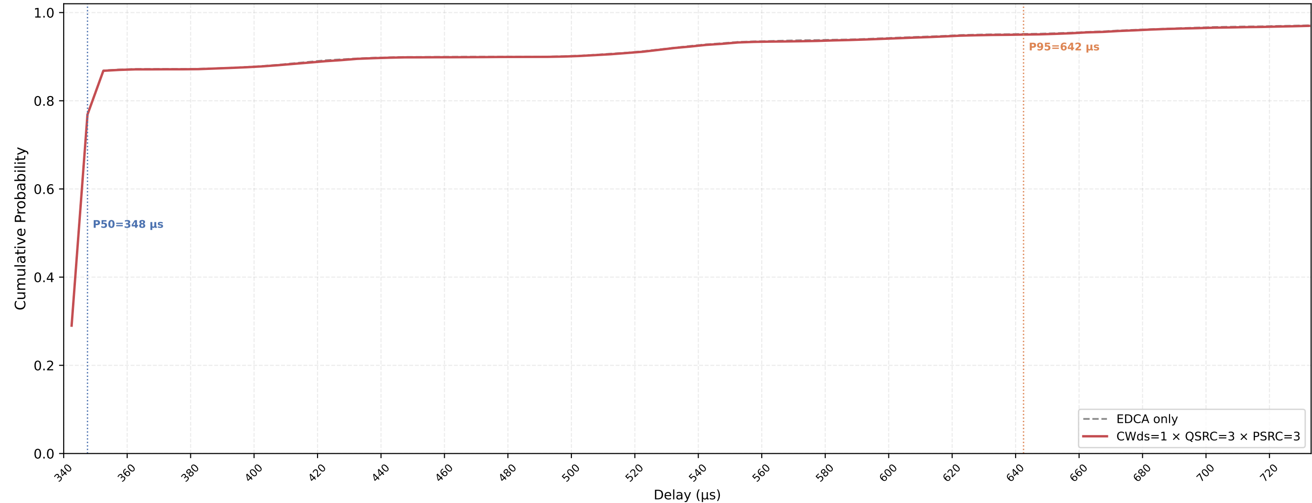
P-EDCA STA VO Delay CDF — CWds=1 × QSRC=3 × PSRC=3 nSta=30, nPedca=30, 0.1Mbps, avg of 10 runs
