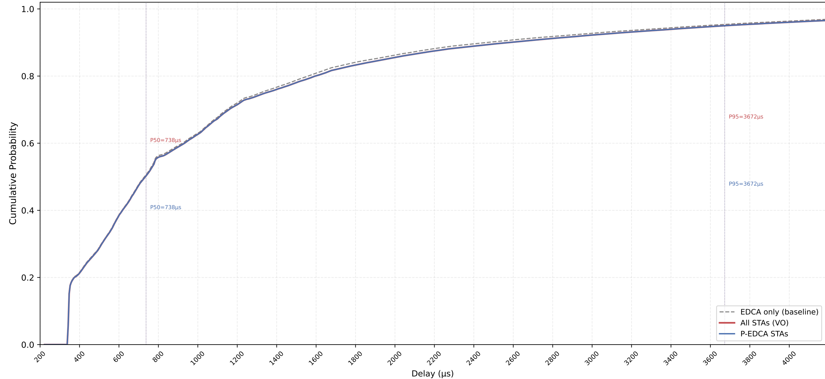
VO Delay CDF — P-EDCA / Legacy / All | CWds=1 × QSRC=4 × PSRC=1 nSta=30, nPedca=30/30, 0.5Mbps, avg of 10 runs
