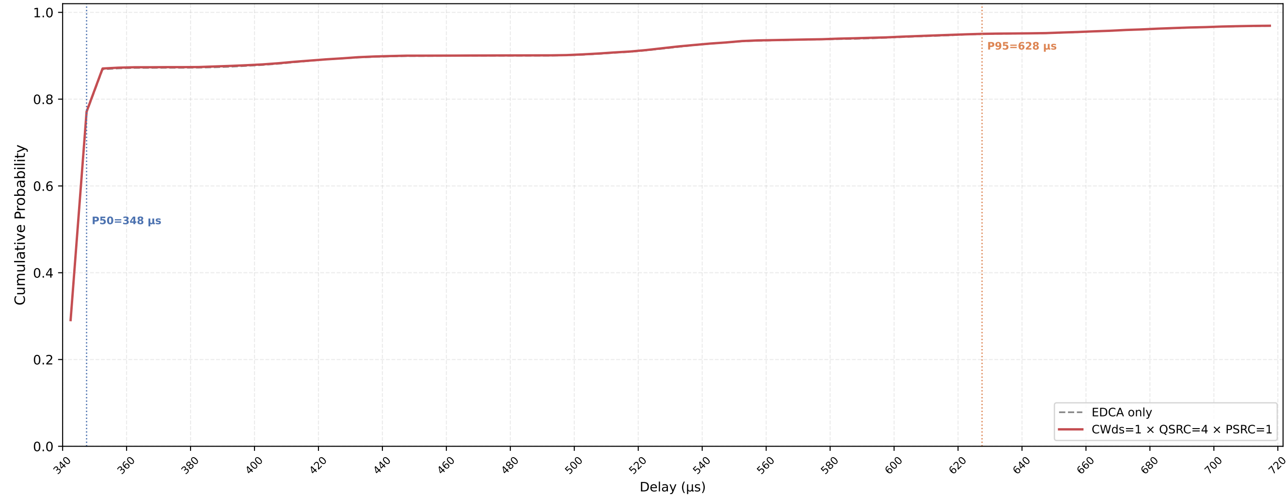
VO (all STAs) Delay CDF — CWds=1 × QSRC=4 × PSRC=1 nSta=30, nPedca=15, 0.1Mbps, avg of 10 runs
