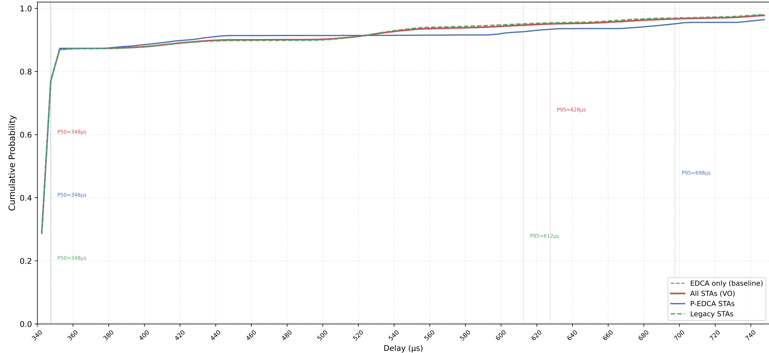
VO Delay CDF — P-EDCA / Legacy / All | CWds=1 × QSRC=4 × PSRC=2 nSta=30, nPedca=5/30, 0.1Mbps, avg of 10 runs
