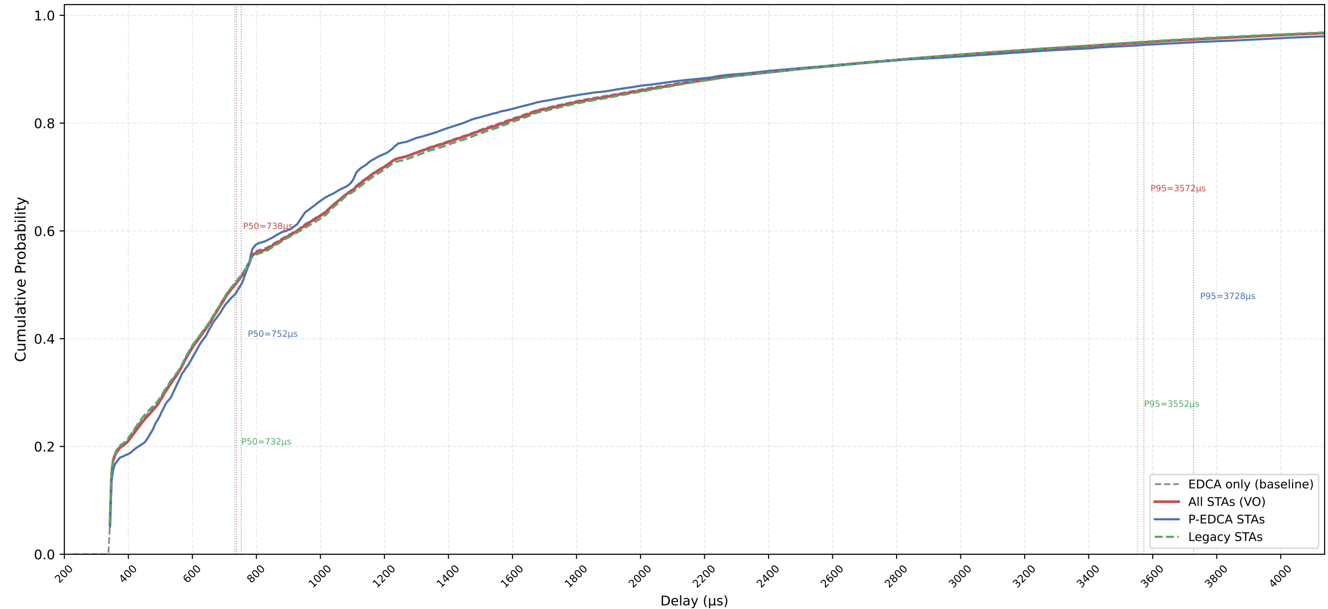
VO Delay CDF — P-EDCA / Legacy / All | CWds=1 × QSRC=4 × PSRC=2 nSta=30, nPedca=5/30, 0.5Mbps, avg of 10 runs
