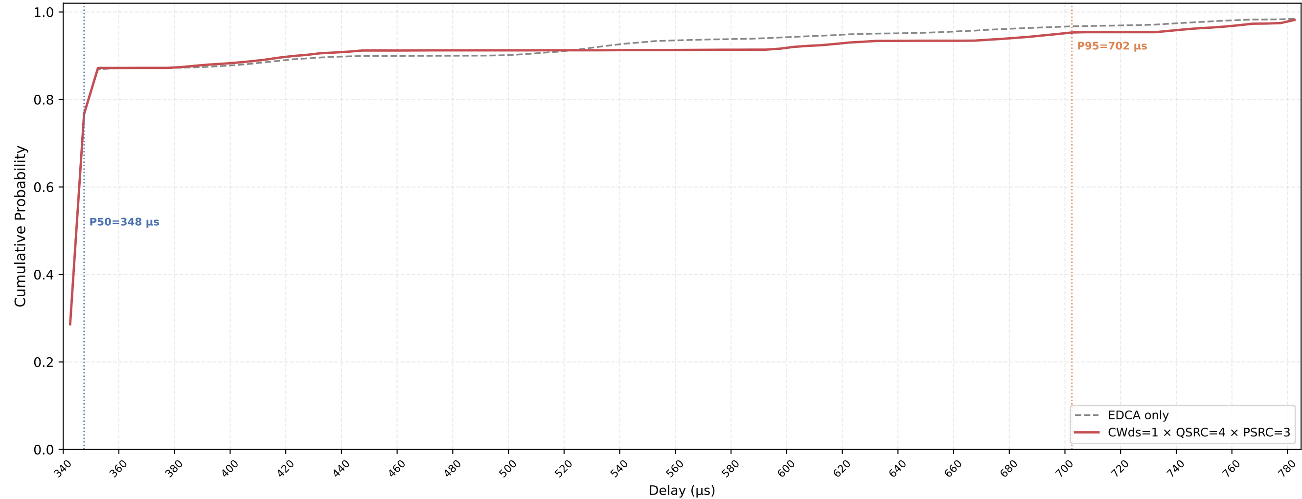
P-EDCA STA VO Delay CDF — CWds=1 × QSRC=4 × PSRC=3 nSta=30, nPedca=5, 0.1Mbps, avg of 10 runs
