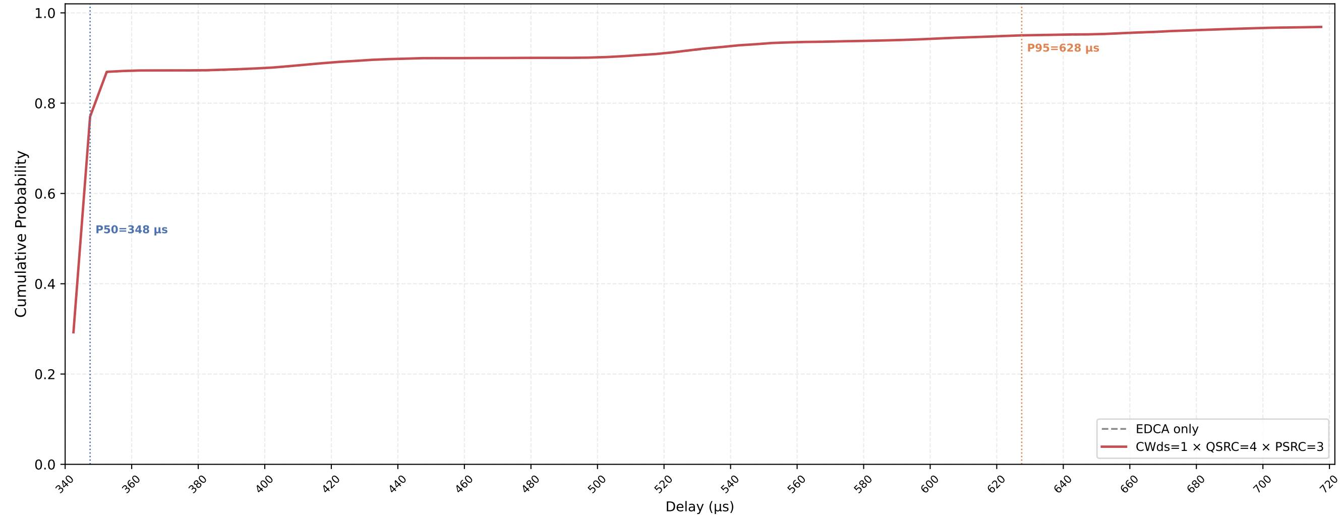
VO (all STAs) Delay CDF — CWds=1 × QSRC=4 × PSRC=3 nSta=30, nPedca=5, 0.1Mbps, avg of 10 runs
