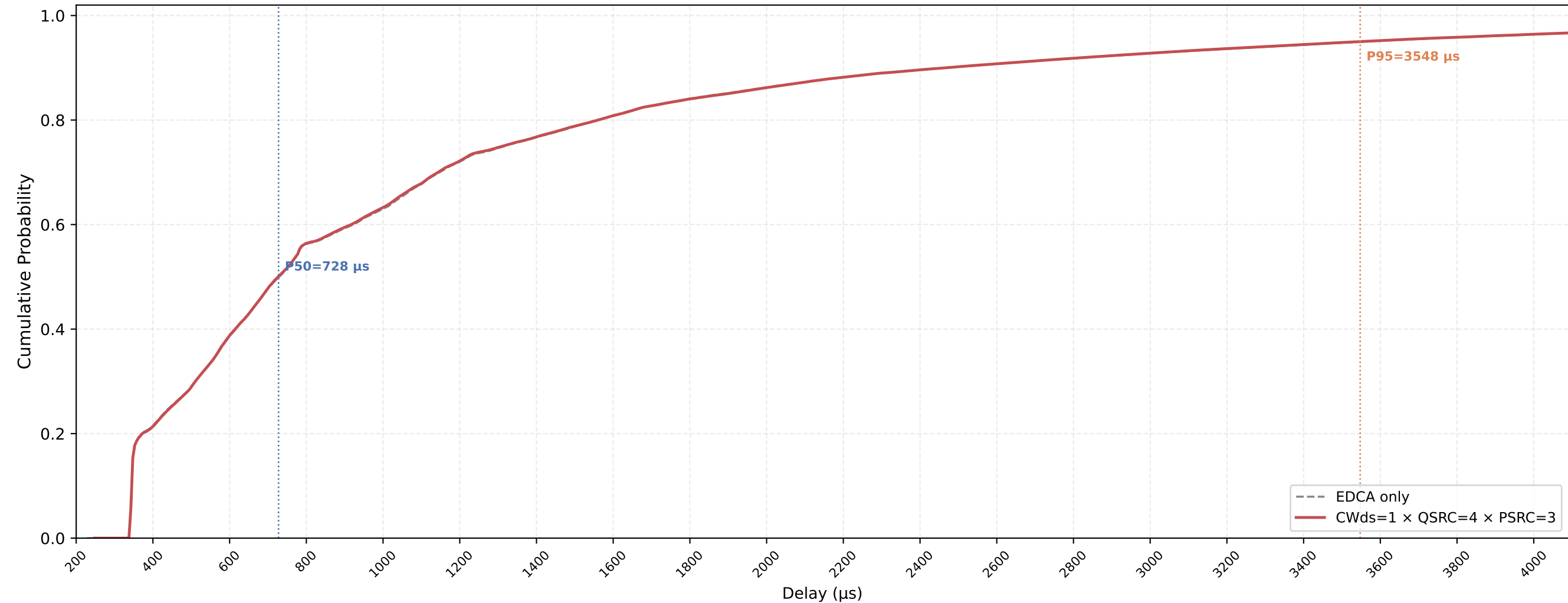
VO (all STAs) Delay CDF — CWds=1 × QSRC=4 × PSRC=3 nSta=30, nPedca=5, 0.5Mbps, avg of 10 runs
