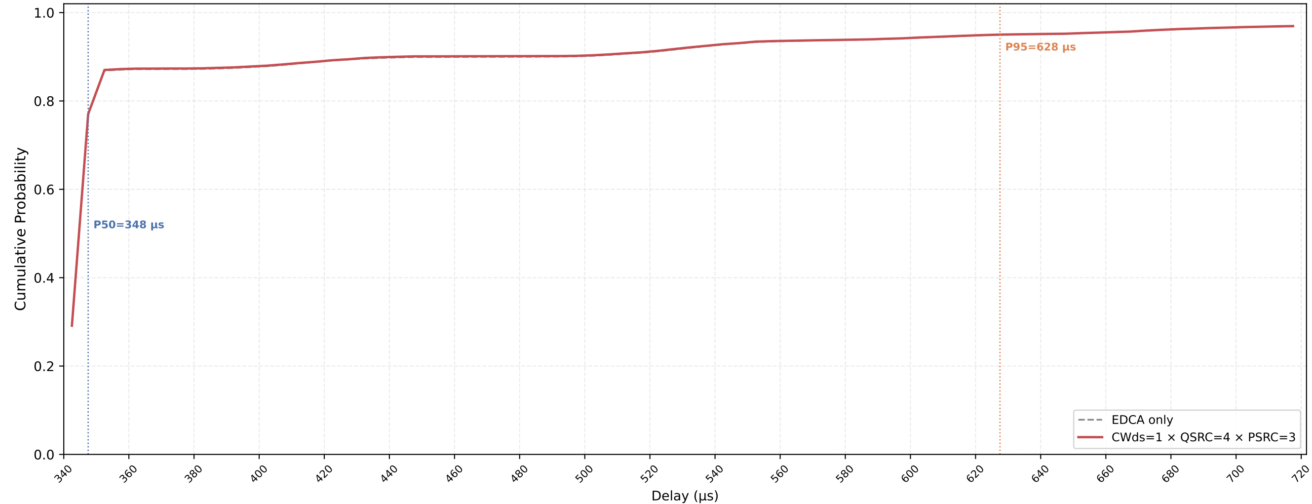
VO (all STAs) Delay CDF — CWds=1 × QSRC=4 × PSRC=3 nSta=30, nPedca=15, 0.1Mbps, avg of 10 runs
