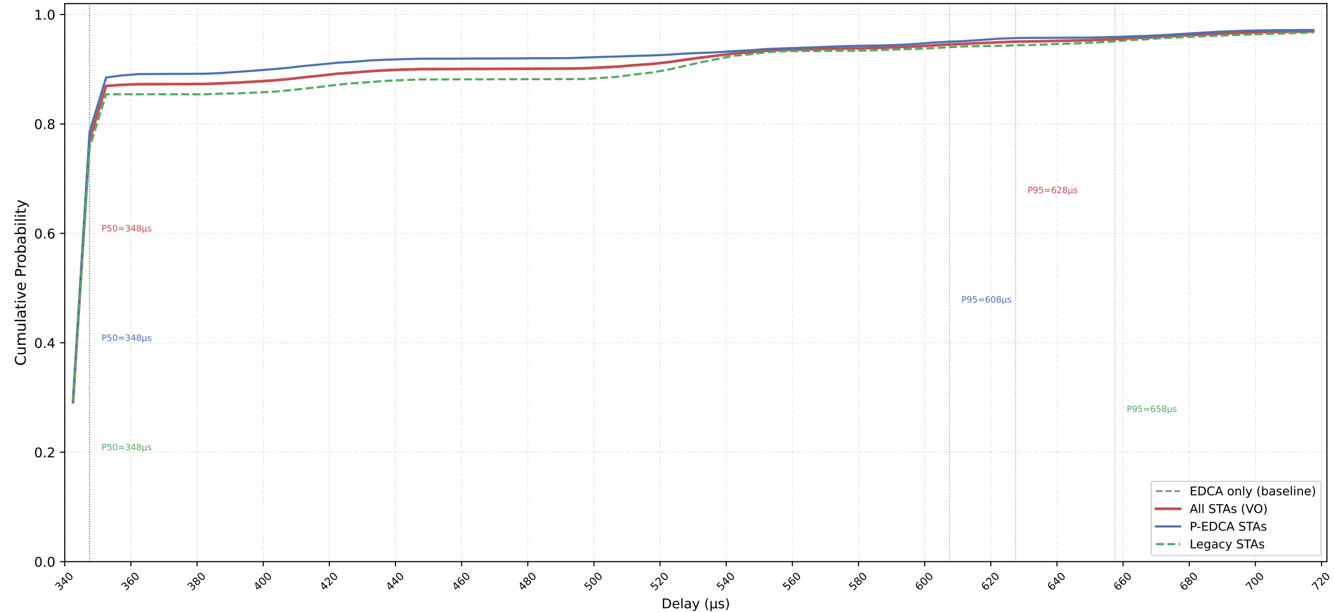
VO Delay CDF — P-EDCA / Legacy / All | CWds=1 × QSRC=5 × PSRC=1 nSta=30, nPedca=15/30, 0.1Mbps, avg of 10 runs
