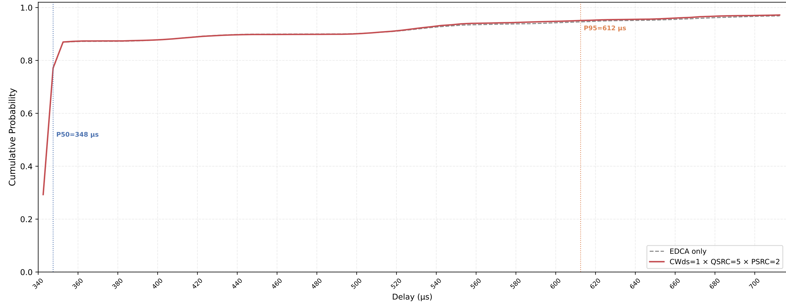
Legacy STA VO Delay CDF — CWds=1 × QSRC=5 × PSRC=2 nSta=30, nPedca=5, 0.1Mbps, avg of 10 runs
