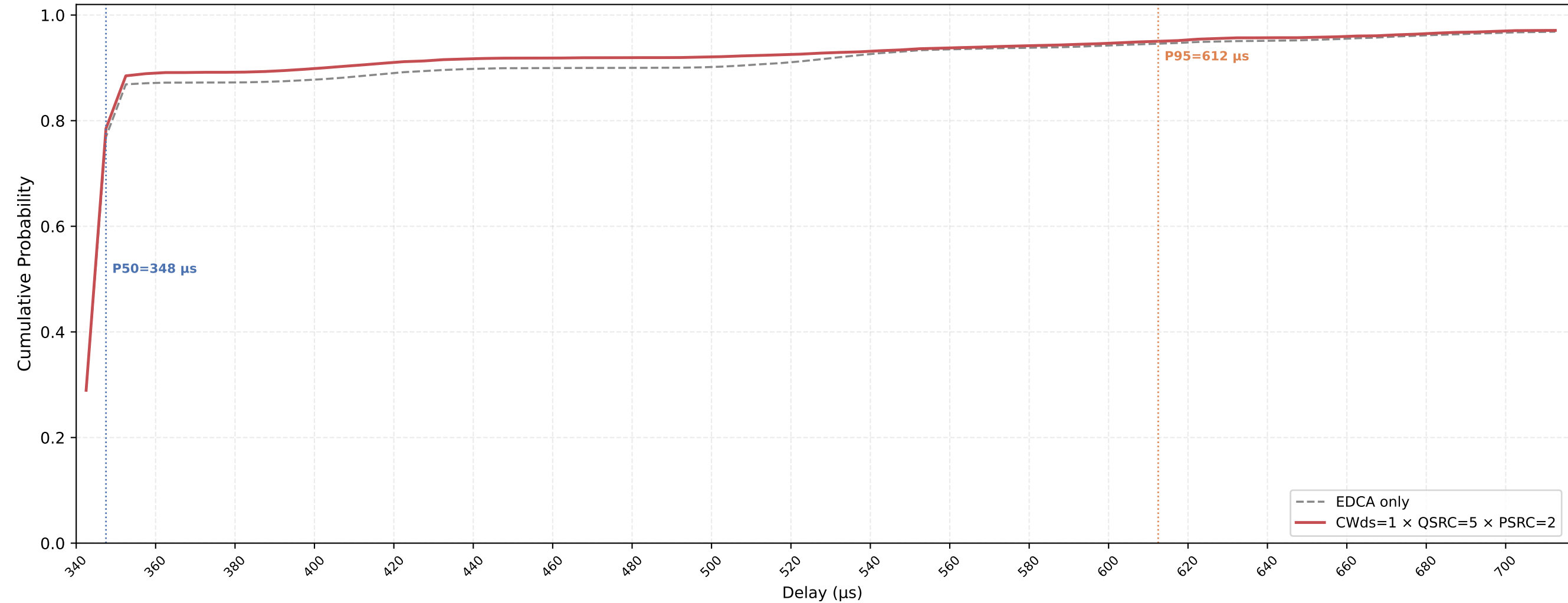
P-EDCA STA VO Delay CDF — CWds=1 × QSRC=5 × PSRC=2 nSta=30, nPedca=15, 0.1Mbps, avg of 10 runs
