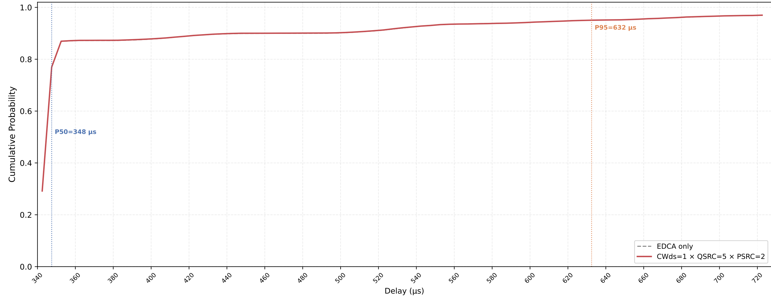
P-EDCA STA VO Delay CDF — CWds=1 × QSRC=5 × PSRC=2 nSta=30, nPedca=30, 0.1Mbps, avg of 10 runs
