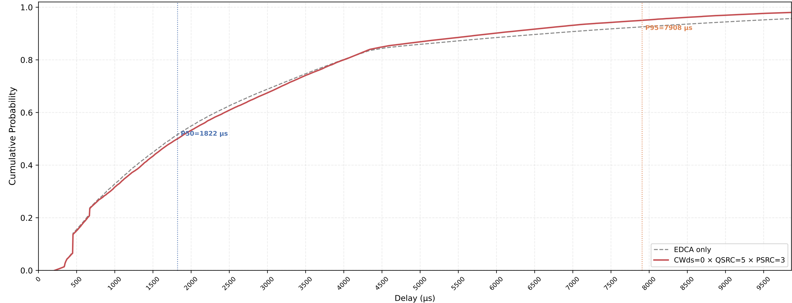
P-EDCA STA VO Delay CDF — CWds=0 × QSRC=5 × PSRC=3 nSta=30, nPedca=5, 1Mbps, avg of 10 runs
