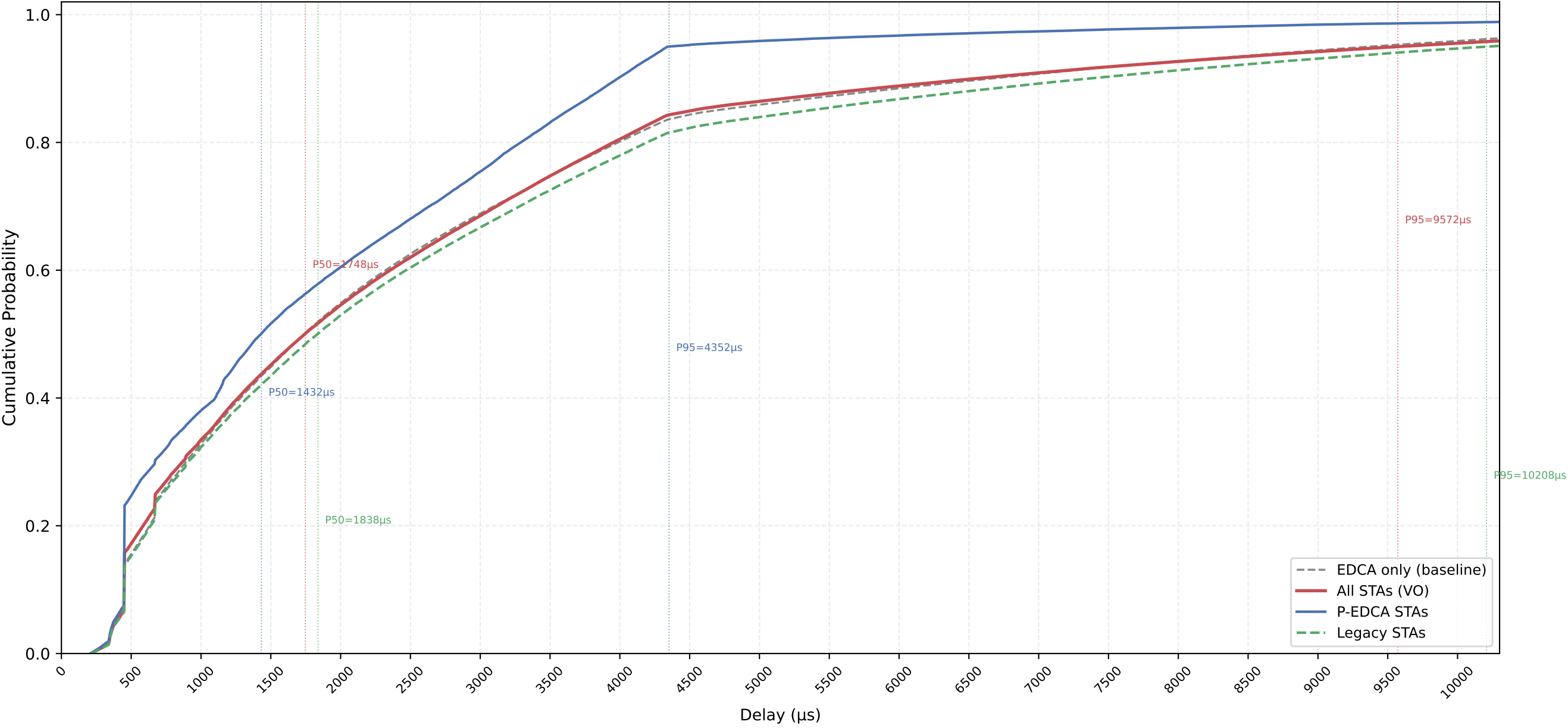
VO Delay CDF — P-EDCA / Legacy / All | CWds=1 × QSRC=2 × PSRC=2 nSta=30, nPedca=5/30, 1Mbps, avg of 10 runs
