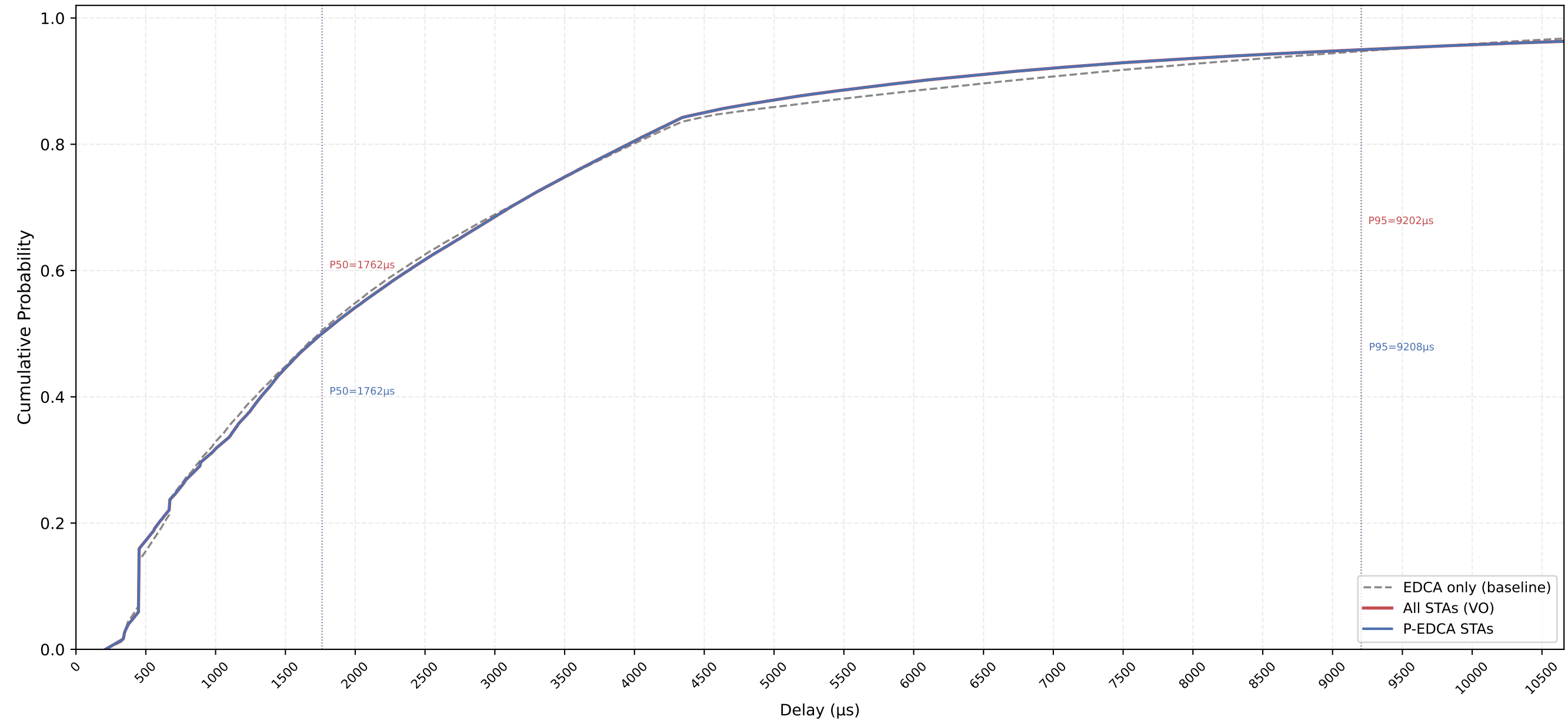
VO Delay CDF — P-EDCA / Legacy / All | CWds=1 × QSRC=3 × PSRC=3 nSta=30, nPedca=30/30, 1Mbps, avg of 10 runs
