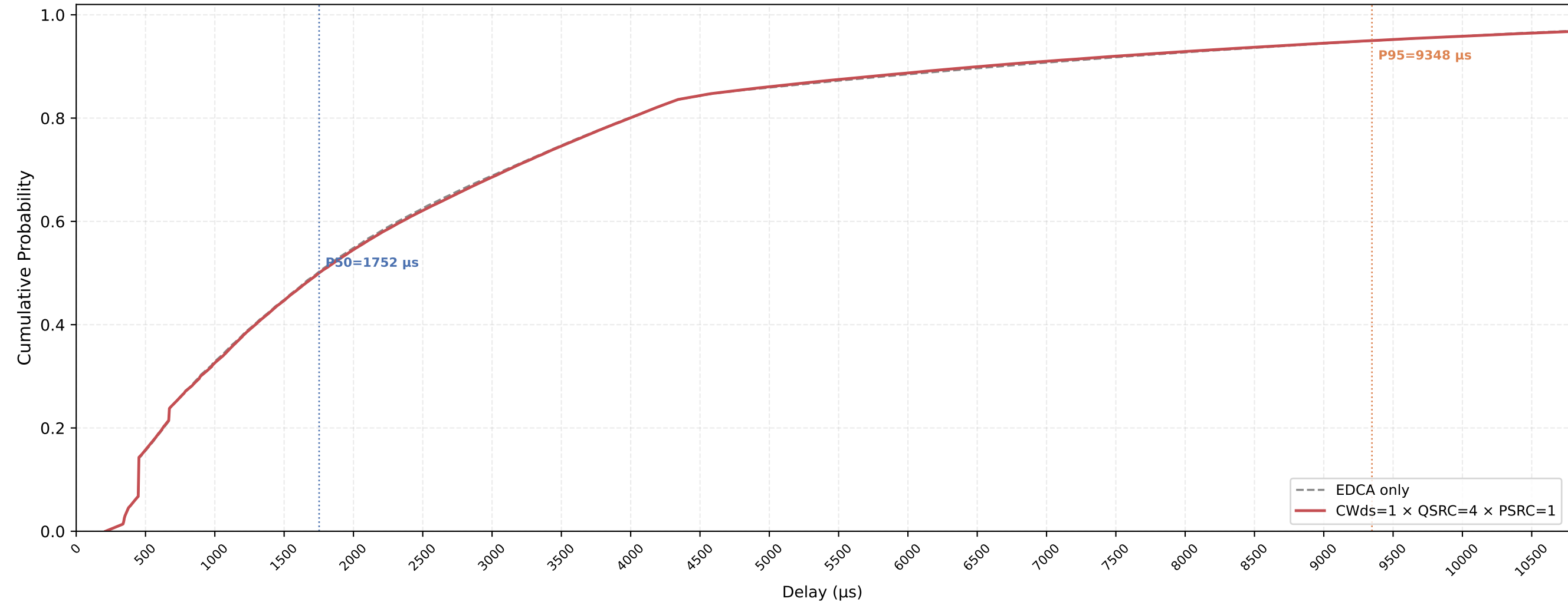
VO (all STAs) Delay CDF — CWds=1 × QSRC=4 × PSRC=1 nSta=30, nPedca=5, 1Mbps, avg of 10 runs
