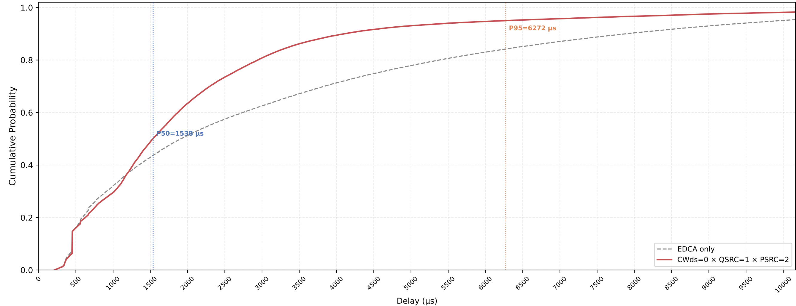
P-EDCA STA VO Delay CDF — CWds=0 × QSRC=1 × PSRC=2 nSta=30, nPedca=5, 1Mbps, avg of 10 runs
