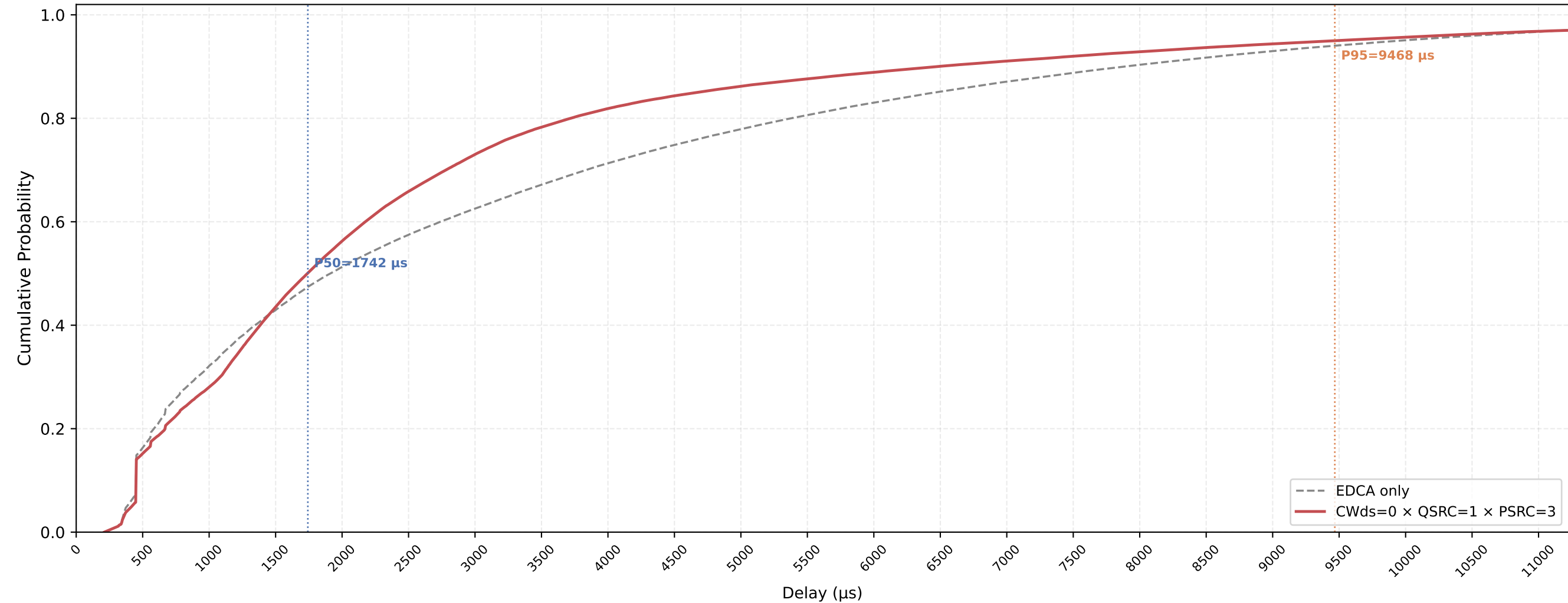
P-EDCA STA VO Delay CDF — CWds=0 × QSRC=1 × PSRC=3 nSta=30, nPedca=15, 1Mbps, avg of 10 runs
