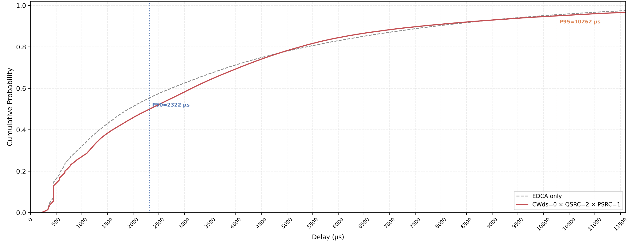
VO (all STAs) Delay CDF — CWds=0 × QSRC=2 × PSRC=1 nSta=30, nPedca=30, 1Mbps, avg of 10 runs
