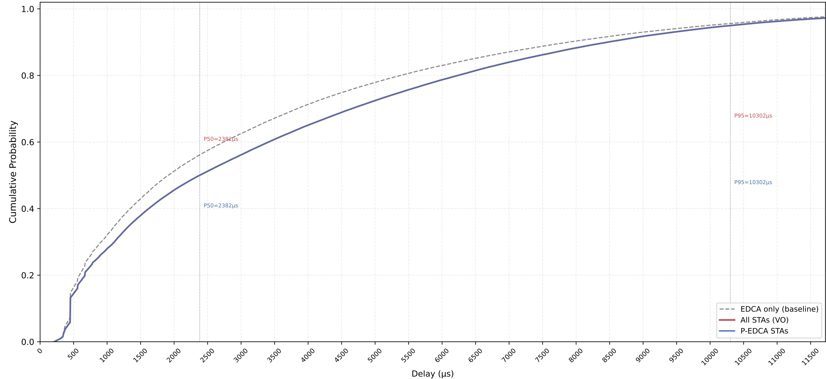
VO Delay CDF — P-EDCA / Legacy / All | CWds=0 × QSRC=4 × PSRC=1 nSta=30, nPedca=30/30, 1Mbps, avg of 10 runs
