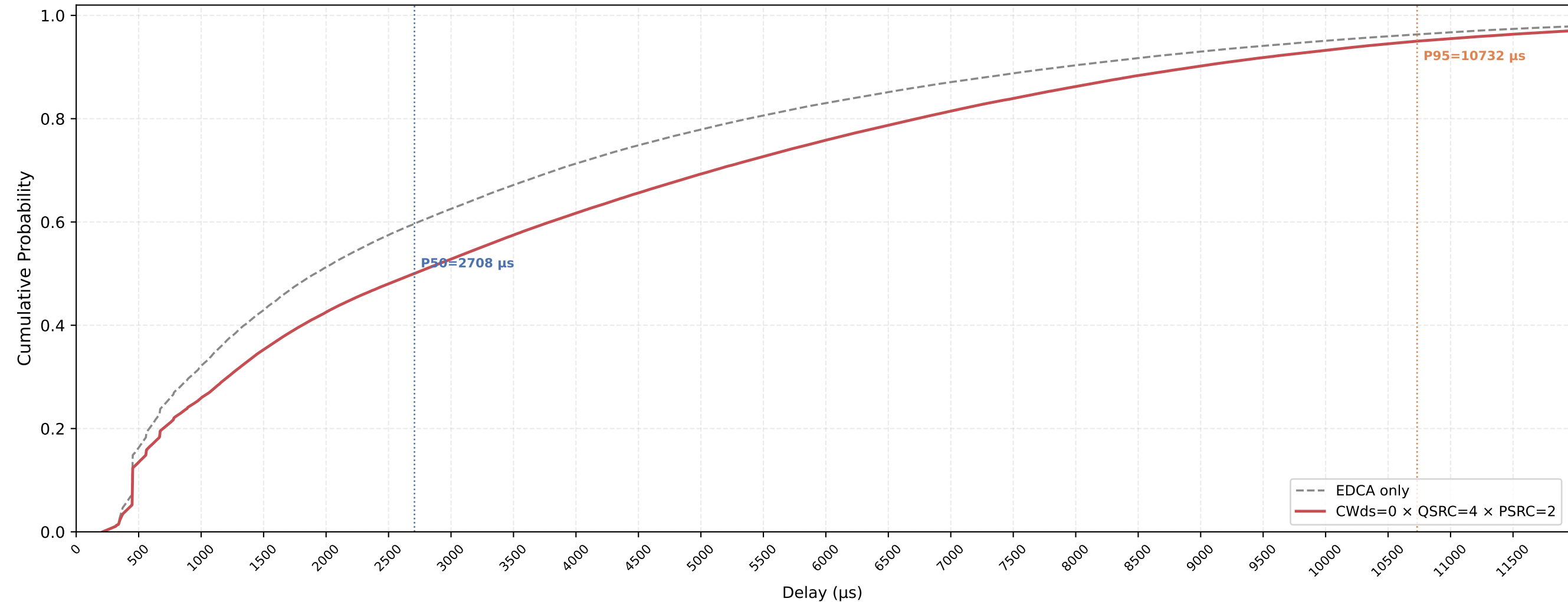
VO (all STAs) Delay CDF — CWds=0 × QSRC=4 × PSRC=2 nSta=30, nPedca=30, 1Mbps, avg of 10 runs
