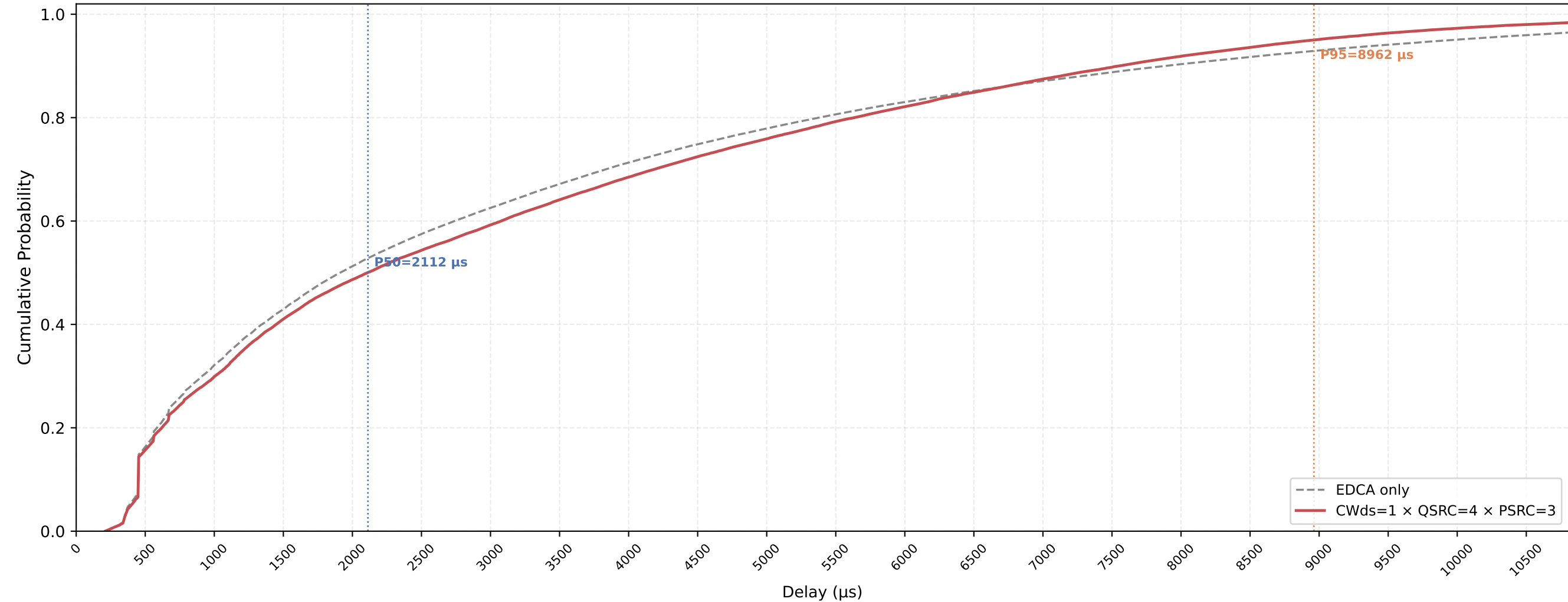
P-EDCA STA VO Delay CDF — CWds=1 × QSRC=4 × PSRC=3 nSta=30, nPedca=5, 1Mbps, avg of 10 runs
