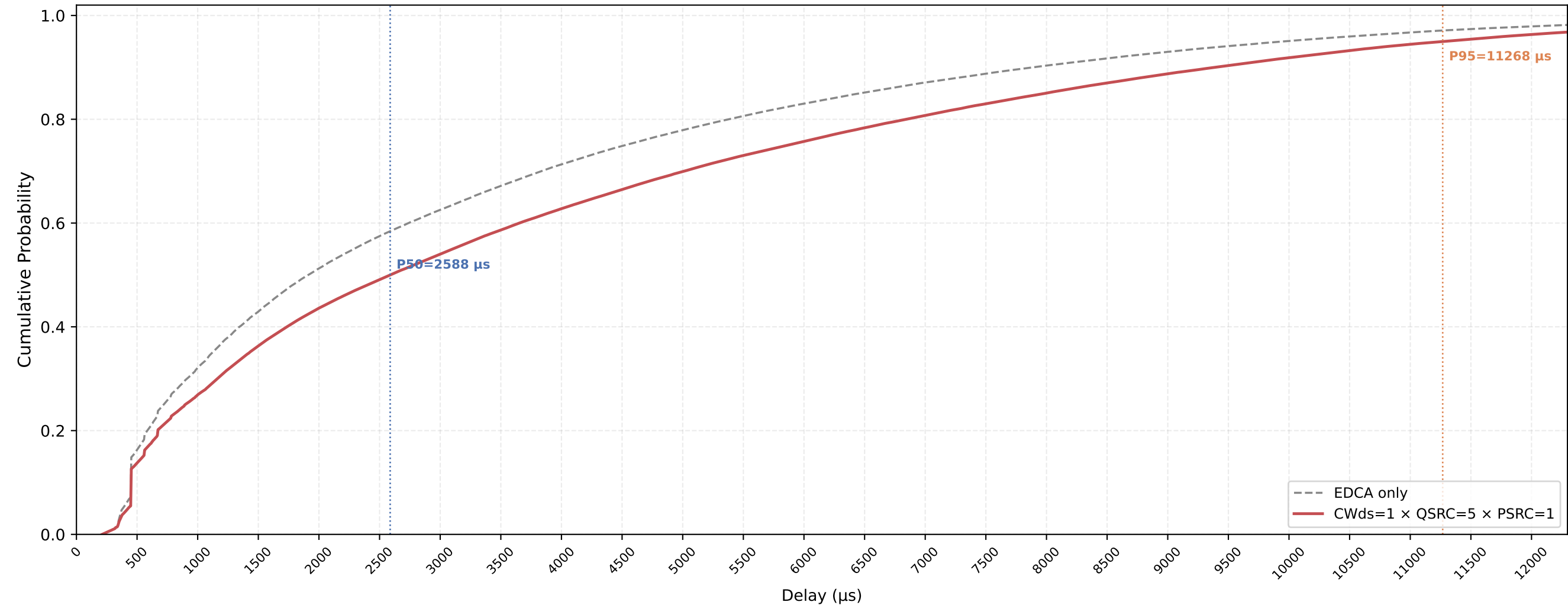
P-EDCA STA VO Delay CDF — CWds=1 × QSRC=5 × PSRC=1 nSta=30, nPedca=30, 1Mbps, avg of 10 runs
