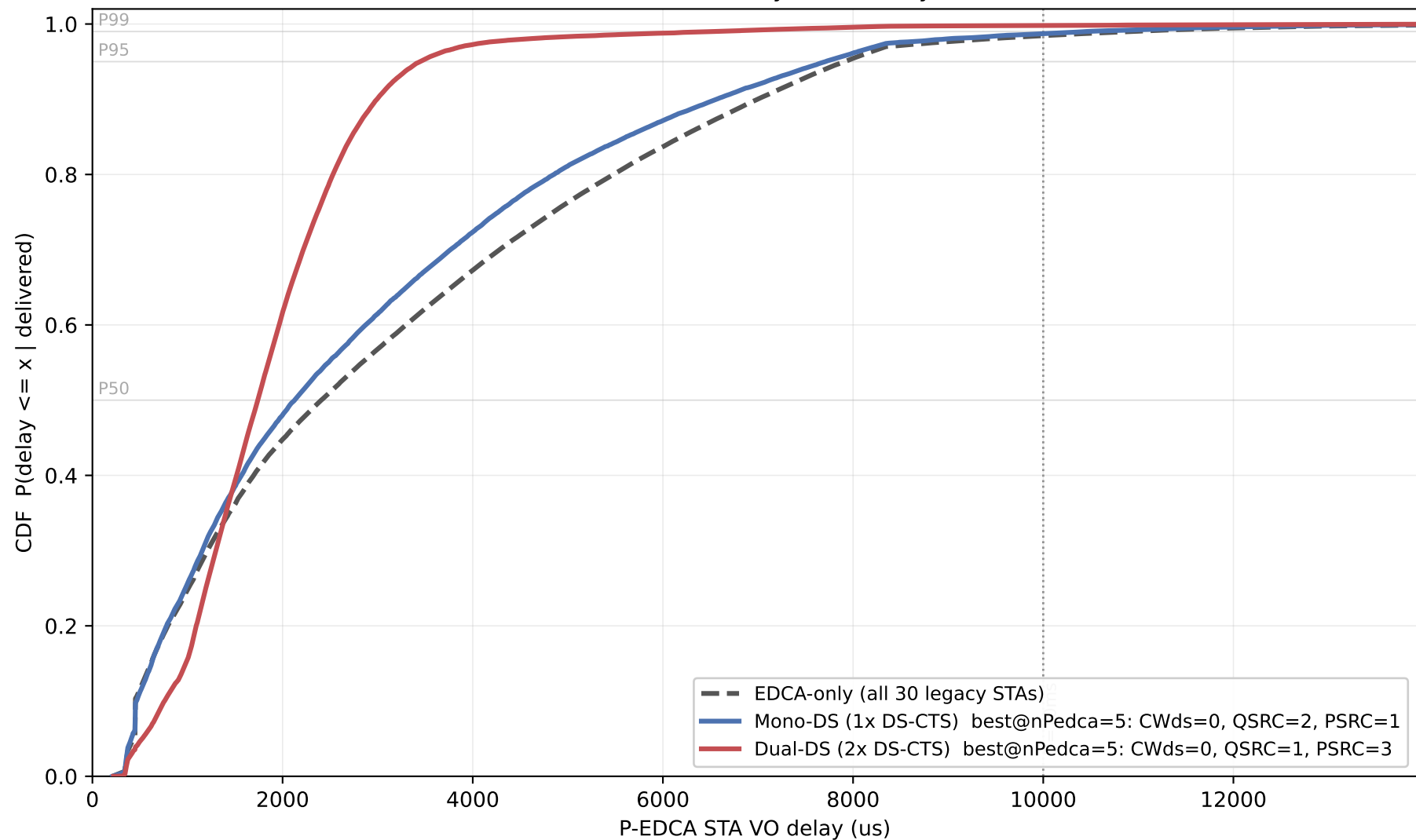
P-EDCA STA Delay CDF at Best Parameters (nPedca=5/30, nSta=30, 1Mbps) curves normalised to 1.0 — delay SHAPE only, loss not shown
