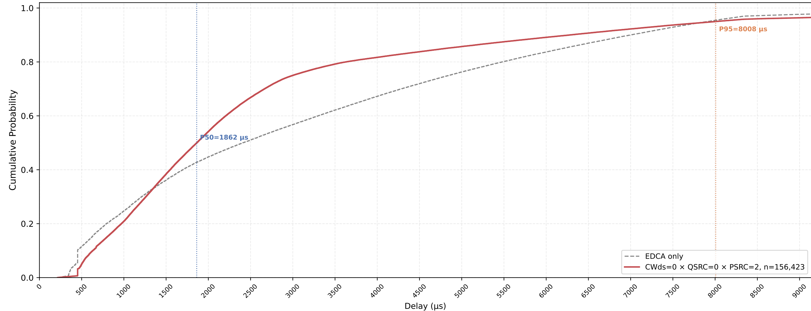
VO (all STAs) Delay CDF — CWds=0 × QSRC=0 × PSRC=2 nSta=30, nPedca=30, 1Mbps, avg of 10 runs
