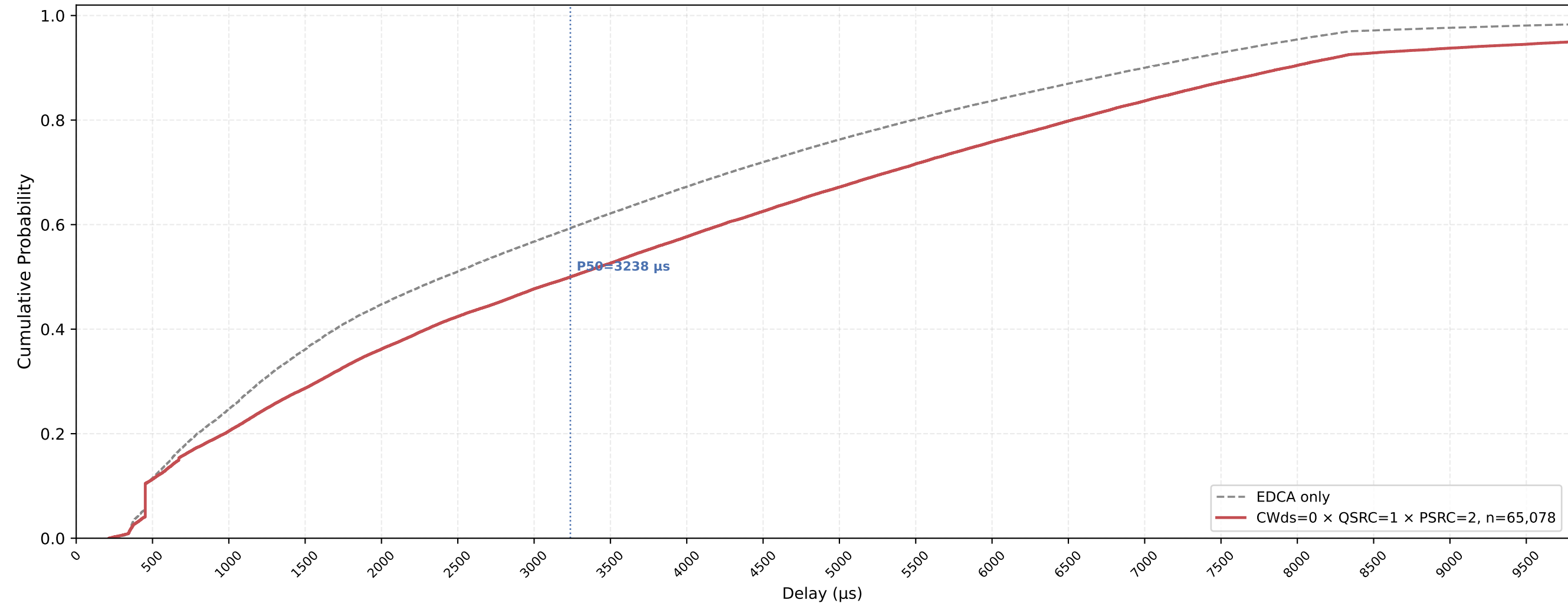
Legacy STA VO Delay CDF — CWds=0 × QSRC=1 × PSRC=2 nSta=30, nPedca=15, 1Mbps, avg of 10 runs
