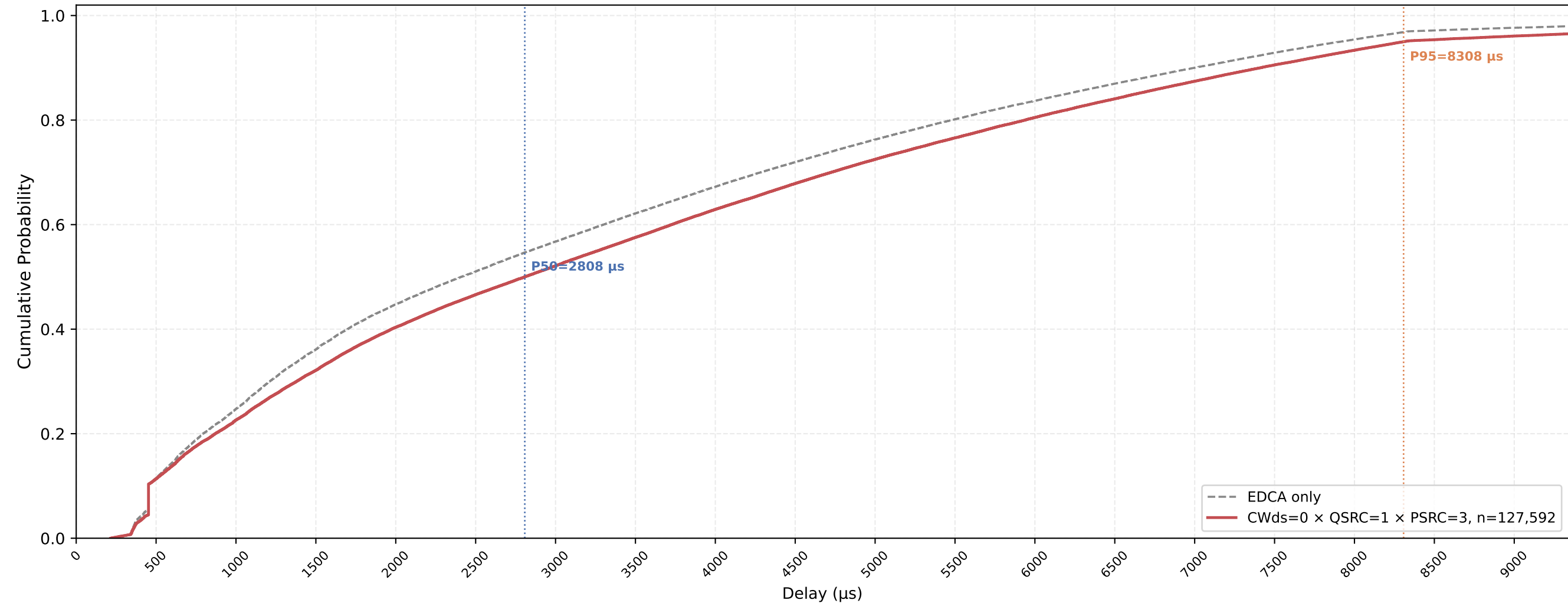
Legacy STA VO Delay CDF — CWds=0 × QSRC=1 × PSRC=3 nSta=30, nPedca=5, 1Mbps, avg of 10 runs
