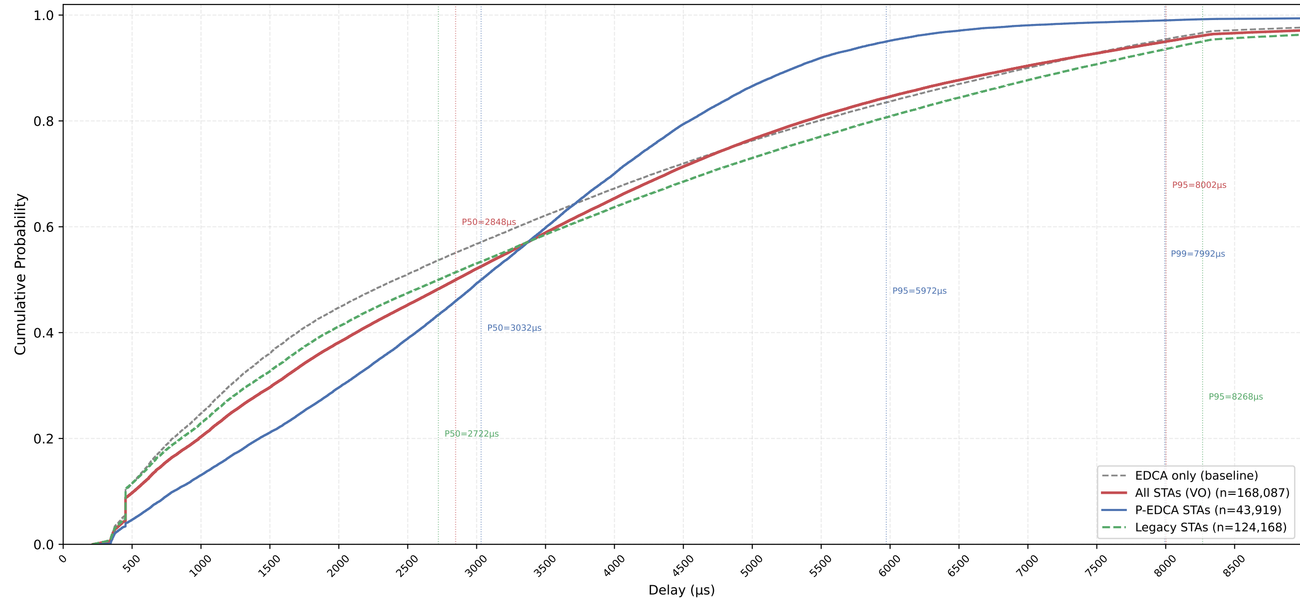
VO Delay CDF — P-EDCA / Legacy / All | CWds=0 × QSRC=2 × PSRC=2 nSta=30, nPedca=5/30, 1Mbps, avg of 10 runs
