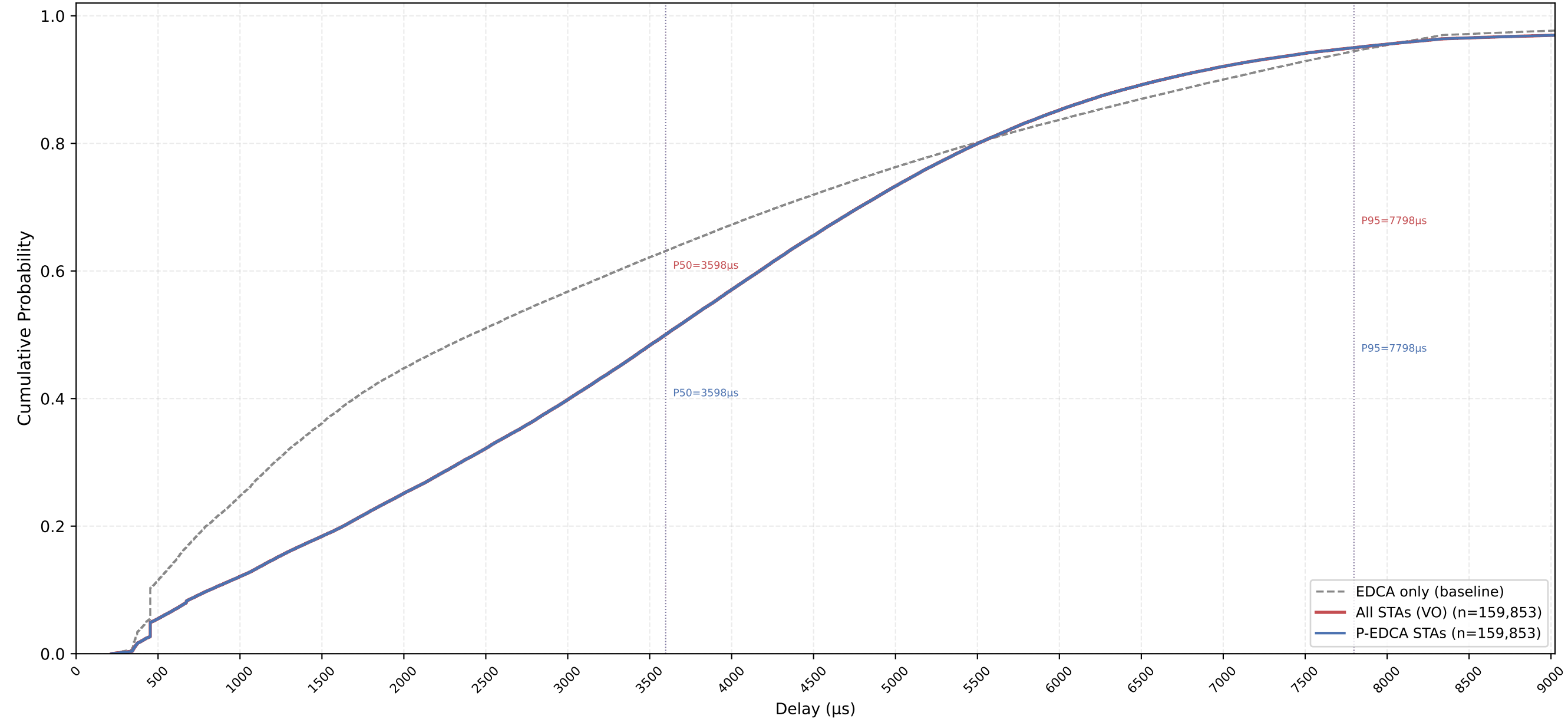
VO Delay CDF — P-EDCA / Legacy / All | CWds=0 × QSRC=2 × PSRC=2 nSta=30, nPedca=30/30, 1Mbps, avg of 10 runs
