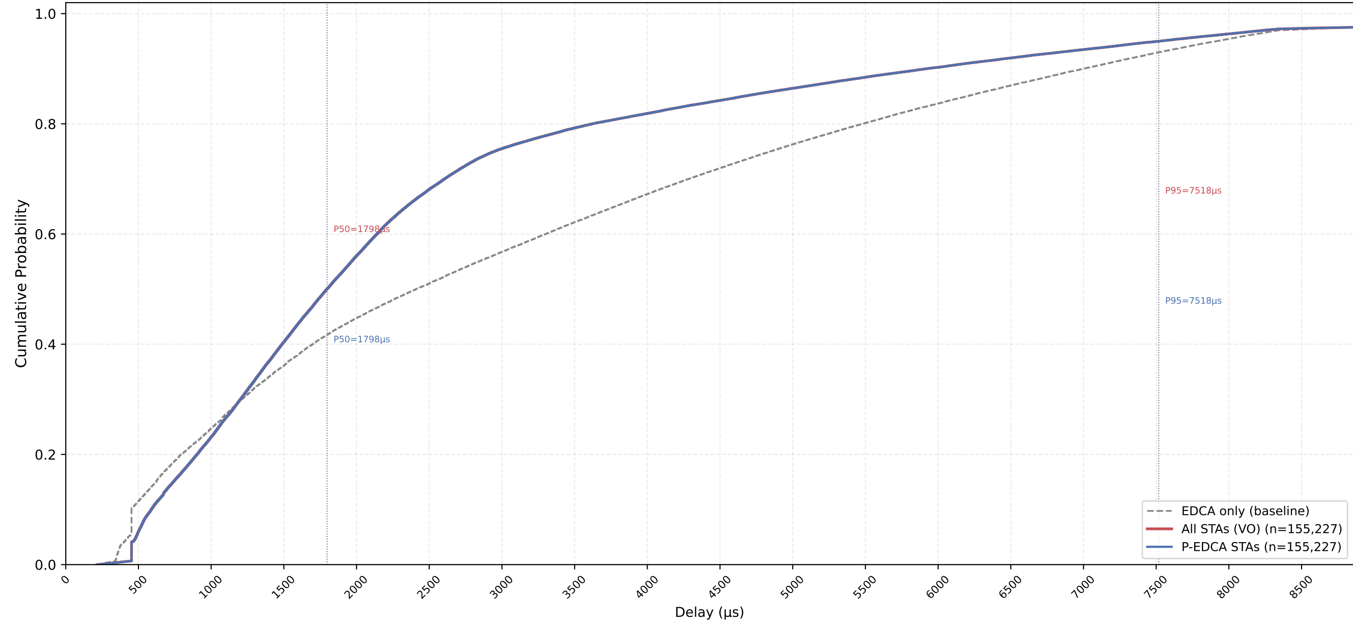
VO Delay CDF — P-EDCA / Legacy / All | CWds=1 × QSRC=0 × PSRC=2 nSta=30, nPedca=30/30, 1Mbps, avg of 10 runs
