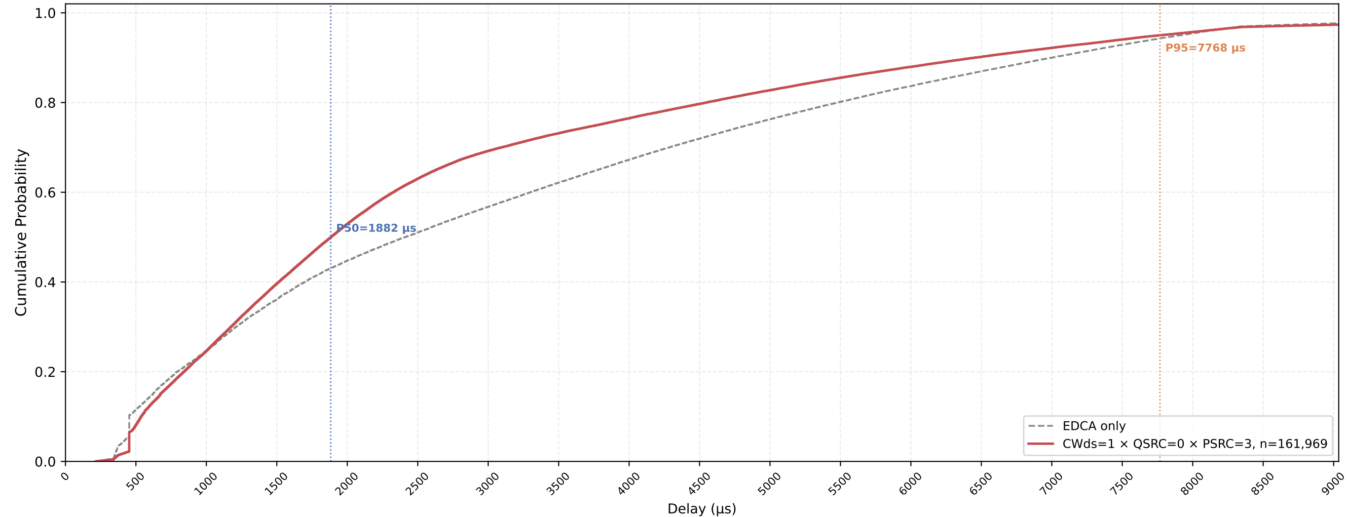
VO (all STAs) Delay CDF — CWds=1 × QSRC=0 × PSRC=3 nSta=30, nPedca=15, 1Mbps, avg of 10 runs
