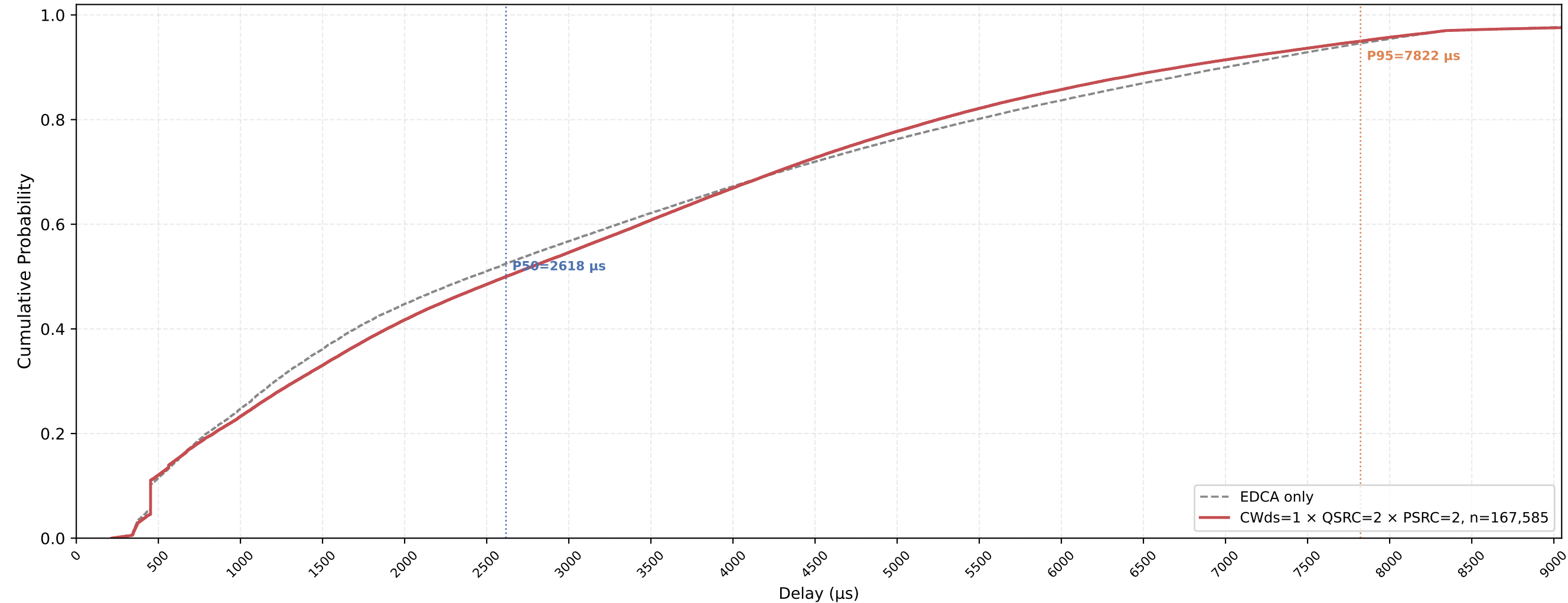
VO (all STAs) Delay CDF — CWds=1 × QSRC=2 × PSRC=2 nSta=30, nPedca=15, 1Mbps, avg of 10 runs
